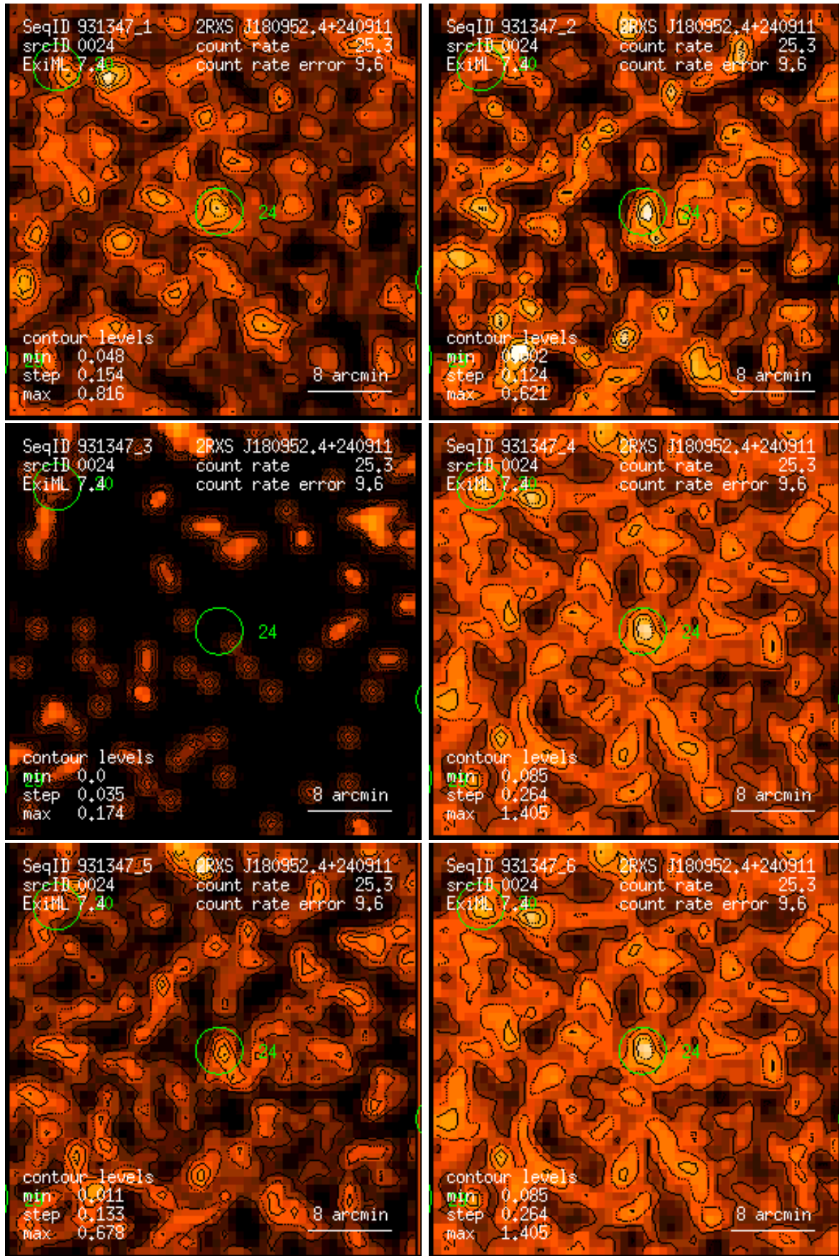
Figure 24: RASS 931347: detection 0024: band rate images, Gaussian filter: (1) PSPC channels 11 – 41, (2) 52 – 90, (3) 91 – 201, (4) 11 – 235, (5) 52 – 201, (6) 11 – 201. Broad band rates in counts/ks. Band rate contour levels in counts/ks/arcmin 2 .
