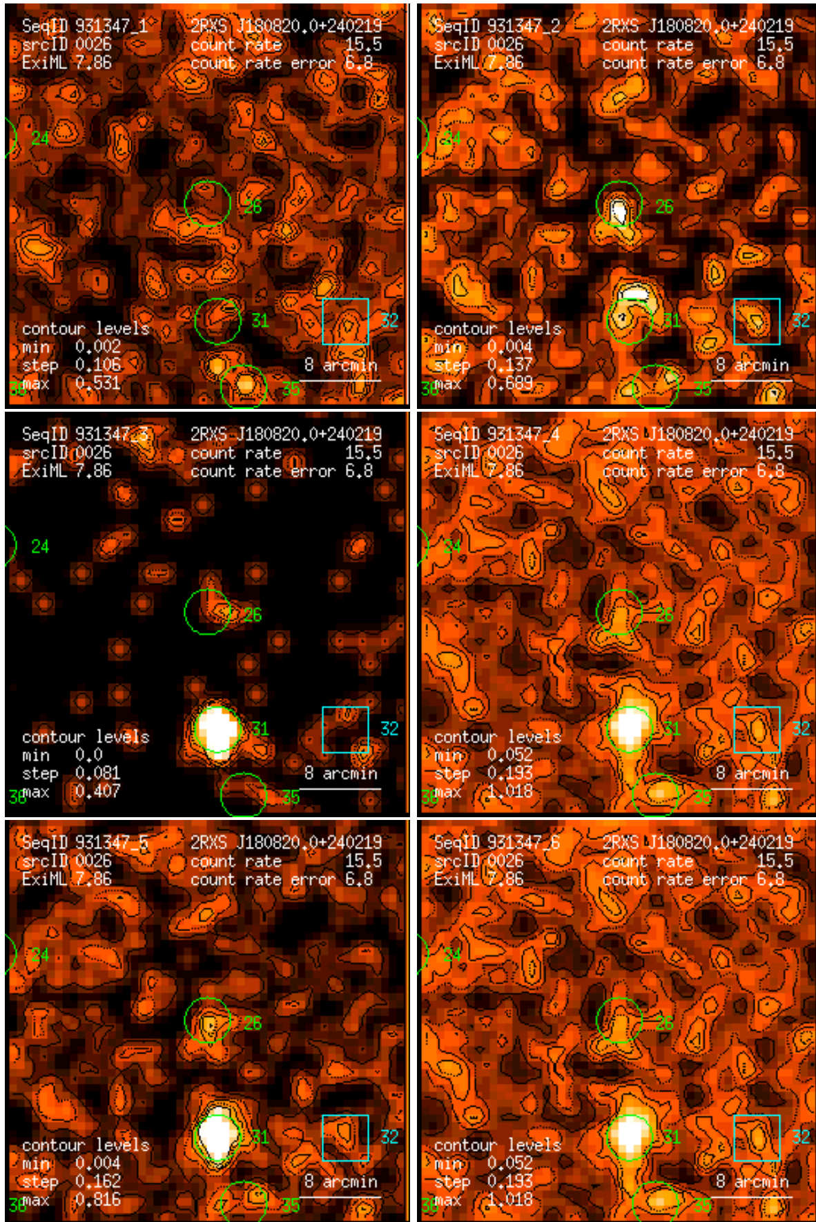
Figure 26: RASS 931347: detection 0026: band rate images, Gaussian filter: (1) PSPC channels 11 – 41, (2) 52 – 90, (3) 91 – 201, (4) 11 – 235, (5) 52 – 201, (6) 11 – 201. Broad band rates in counts/ks. Band rate contour levels in counts/ks/arcmin 2 .
