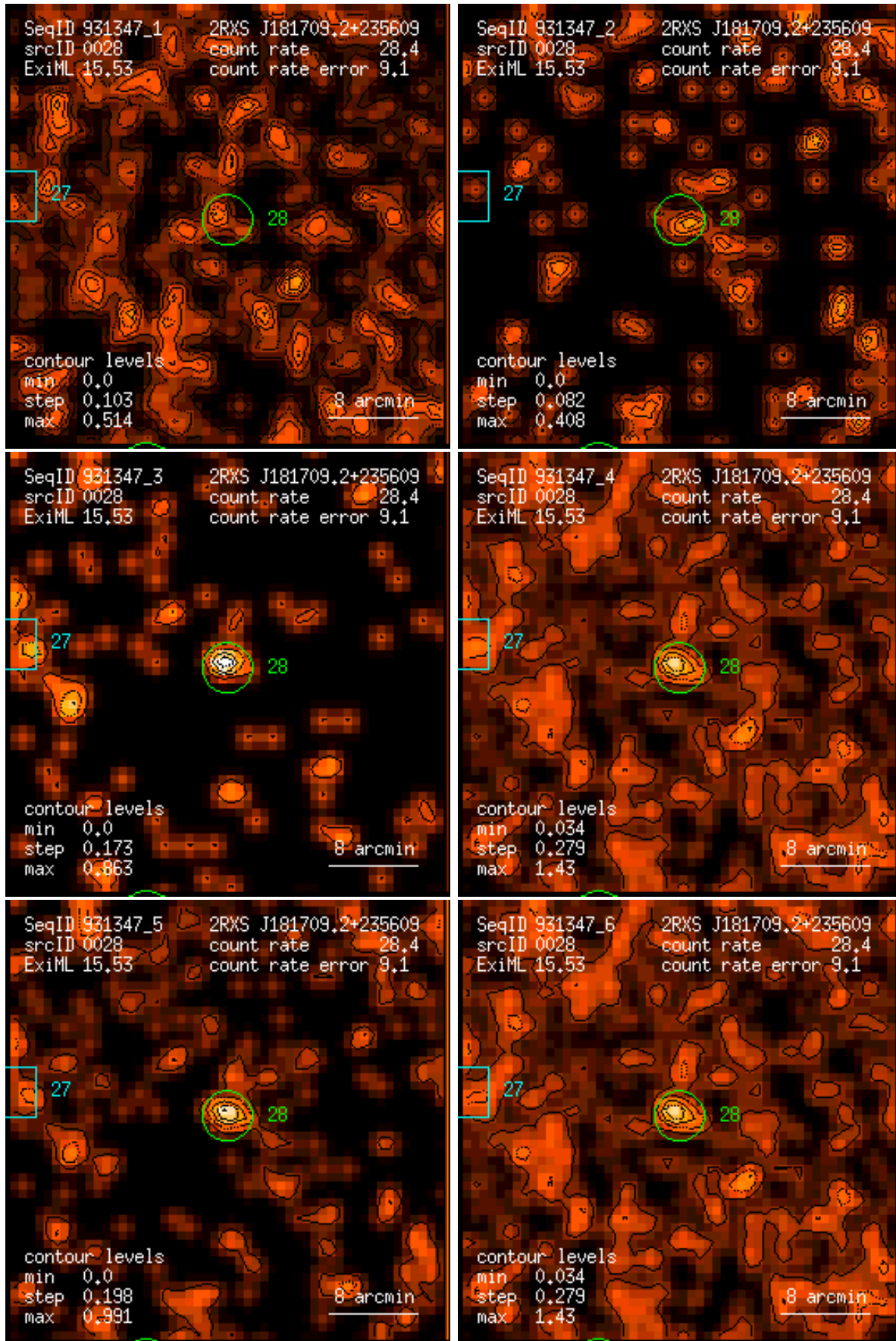
Figure 28: RASS 931347: detection 0028: band rate images, Gaussian filter: (1) PSPC channels 11 – 41, (2) 52 – 90, (3) 91 – 201, (4) 11 – 235, (5) 52 – 201, (6) 11 – 201. Broad band rates in counts/ks. Band rate contour levels in counts/ks/arcmin 2 .
