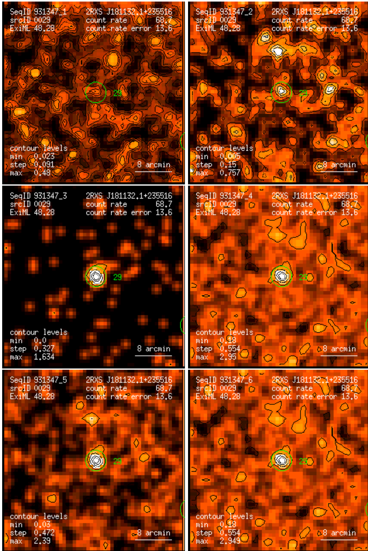
Figure 29: RASS 931347: detection 0029: band rate images, Gaussian filter: (1) PSPC channels 11 – 41, (2) 52 – 90, (3) 91 – 201, (4) 11 – 235, (5) 52 – 201, (6) 11 – 201. Broad band rates in counts/ks. Band rate contour levels in counts/ks/arcmin 2 .
