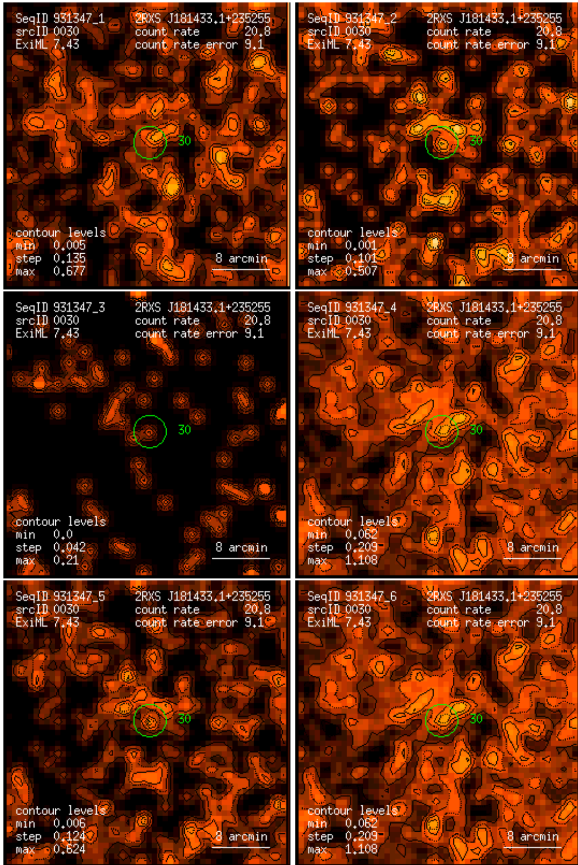
Figure 30: RASS 931347: detection 0030: band rate images, Gaussian filter: (1) PSPC channels 11 – 41, (2) 52 – 90, (3) 91 – 201, (4) 11 – 235, (5) 52 – 201, (6) 11 – 201. Broad band rates in counts/ks. Band rate contour levels in counts/ks/arcmin 2 .
