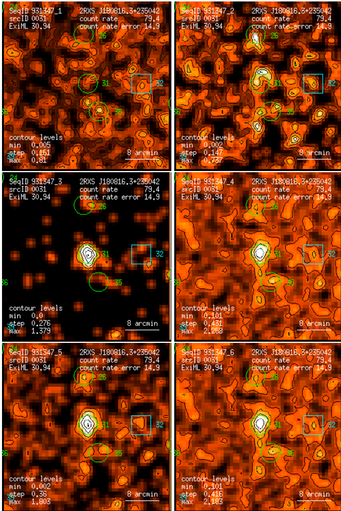
Figure 31: RASS 931347: detection 0031: band rate images, Gaussian filter: (1) PSPC channels 11 – 41, (2) 52 – 90, (3) 91 – 201, (4) 11 – 235, (5) 52 – 201, (6) 11 – 201. Broad band rates in counts/ks. Band rate contour levels in counts/ks/arcmin 2 .
