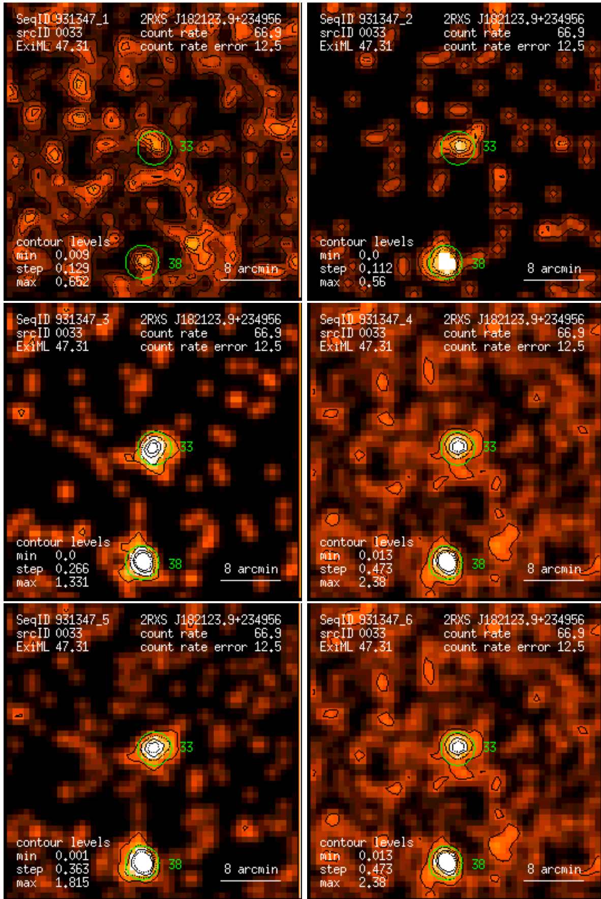
Figure 33: RASS 931347: detection 0033: band rate images, Gaussian filter: (1) PSPC channels 11 – 41, (2) 52 – 90, (3) 91 – 201, (4) 11 – 235, (5) 52 – 201, (6) 11 – 201. Broad band rates in counts/ks. Band rate contour levels in counts/ks/arcmin 2 .
