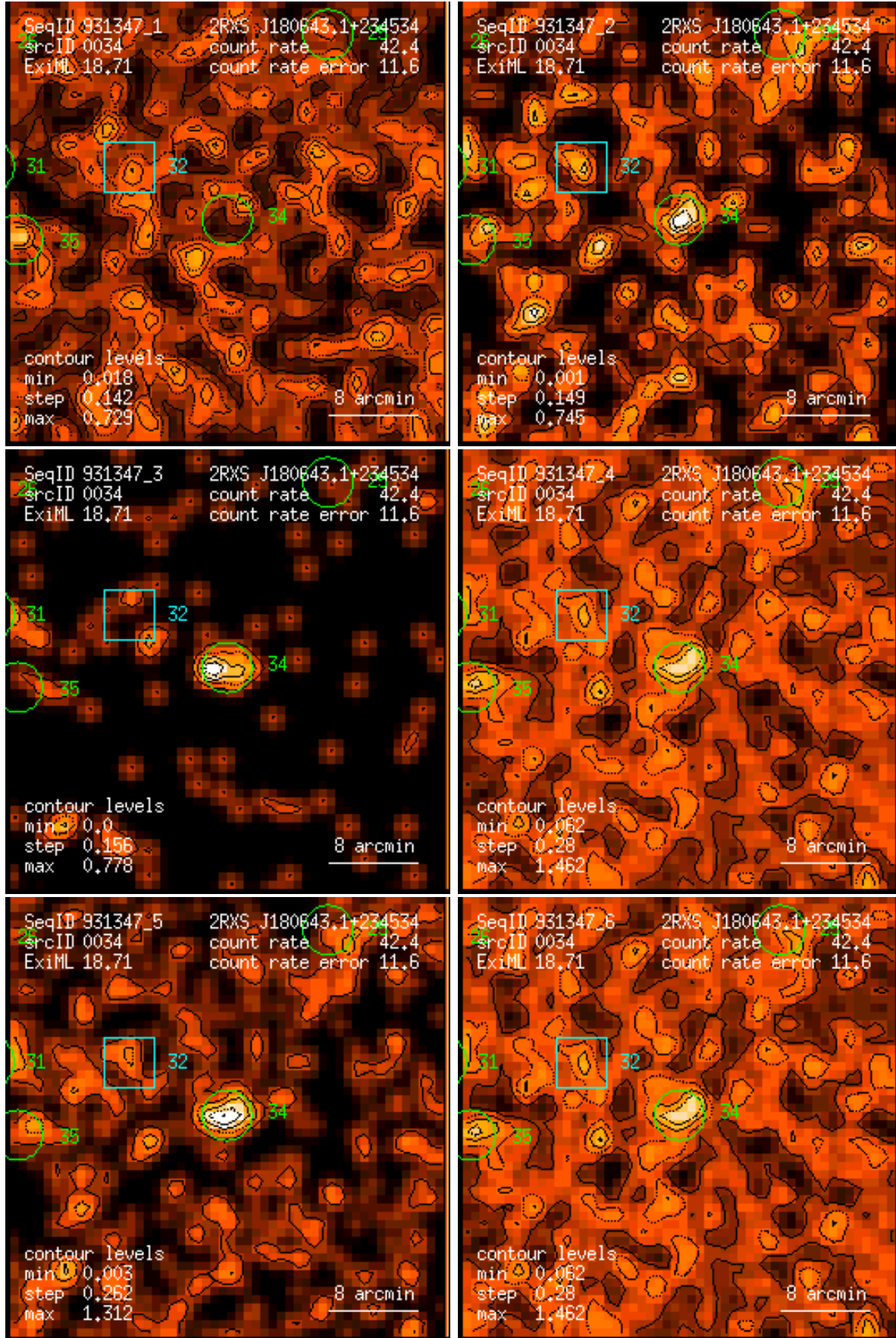
Figure 34: RASS 931347: detection 0034: band rate images, Gaussian filter: (1) PSPC channels 11 – 41, (2) 52 – 90, (3) 91 – 201, (4) 11 – 235, (5) 52 – 201, (6) 11 – 201. Broad band rates in counts/ks. Band rate contour levels in counts/ks/arcmin 2 .
