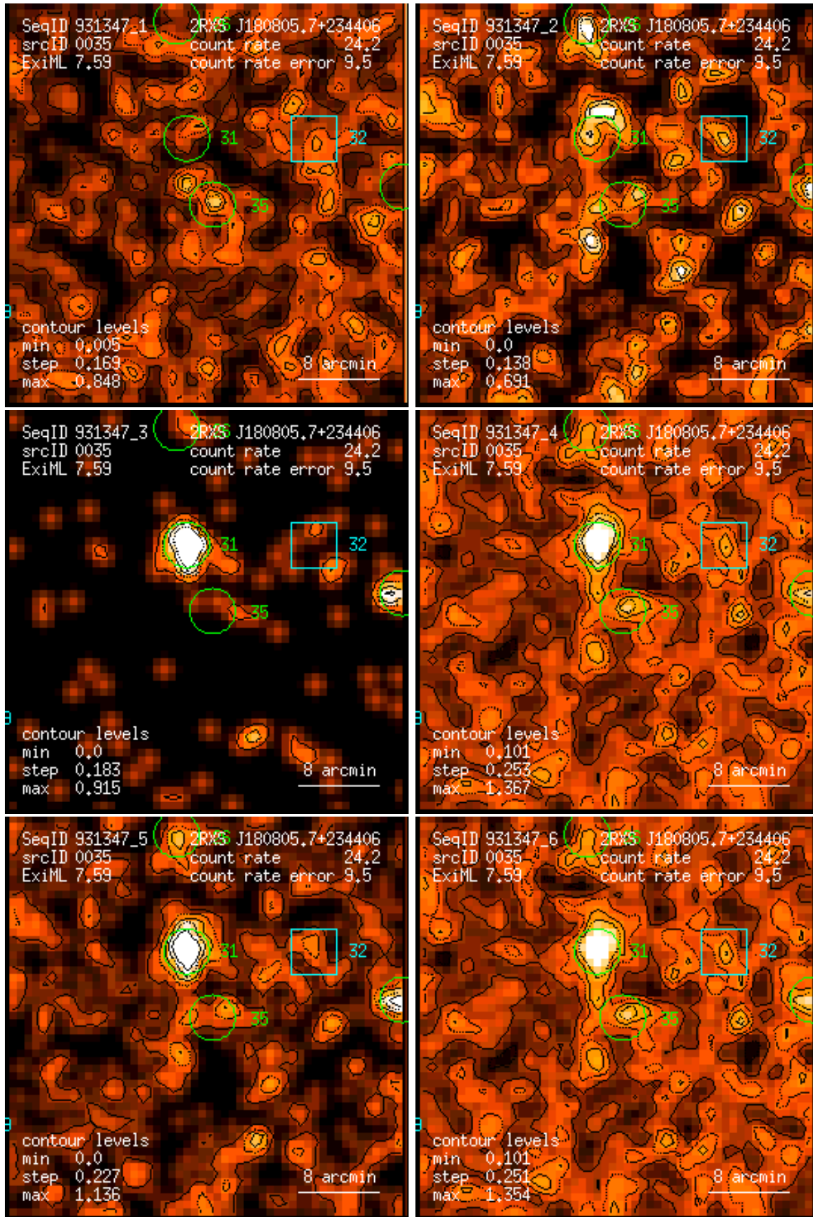
Figure 35: RASS 931347: detection 0035: band rate images, Gaussian filter: (1) PSPC channels 11 – 41, (2) 52 – 90, (3) 91 – 201, (4) 11 – 235, (5) 52 – 201, (6) 11 – 201. Broad band rates in counts/ks. Band rate contour levels in counts/ks/arcmin 2 .
