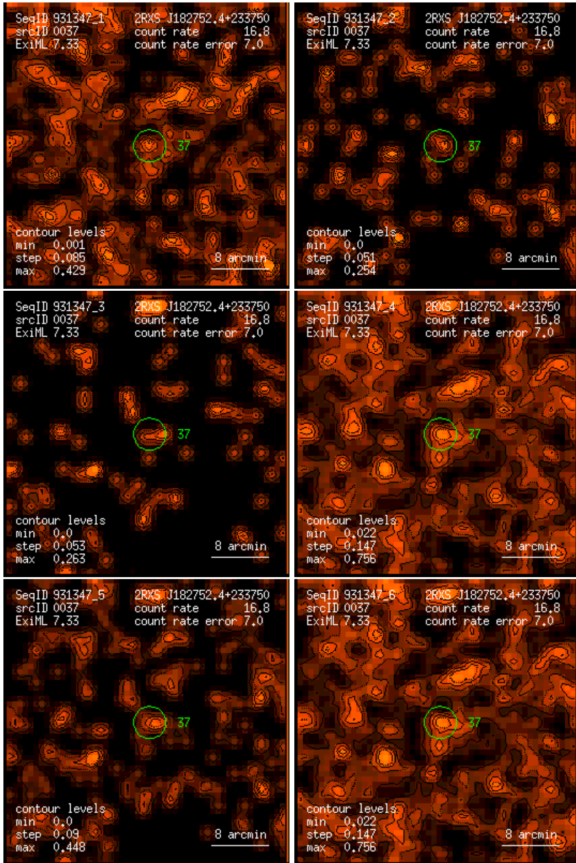
Figure 37: RASS 931347: detection 0037: band rate images, Gaussian filter: (1) PSPC channels 11 – 41, (2) 52 – 90, (3) 91 – 201, (4) 11 – 235, (5) 52 – 201, (6) 11 – 201. Broad band rates in counts/ks. Band rate contour levels in counts/ks/arcmin 2 .
