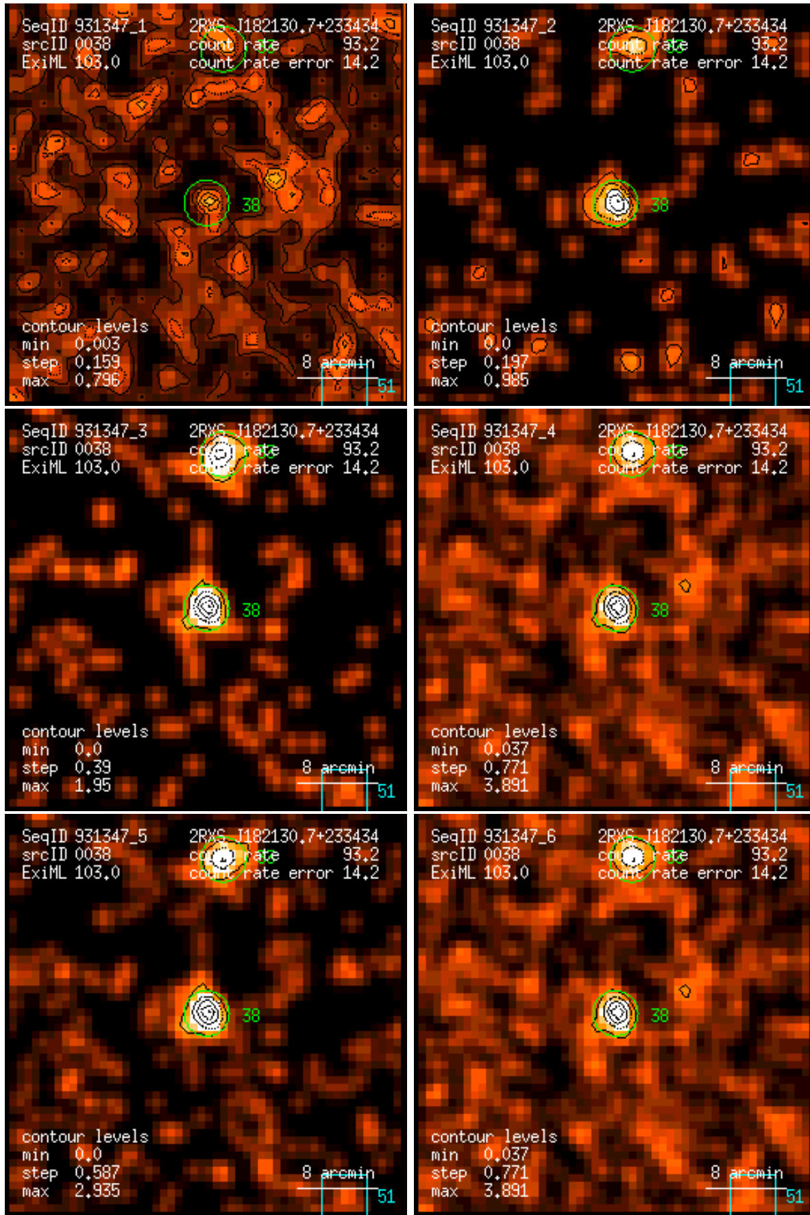
Figure 38: RASS 931347: detection 0038: band rate images, Gaussian filter: (1) PSPC channels 11 – 41, (2) 52 – 90, (3) 91 – 201, (4) 11 – 235, (5) 52 – 201, (6) 11 – 201. Broad band rates in counts/ks. Band rate contour levels in counts/ks/arcmin 2 .
