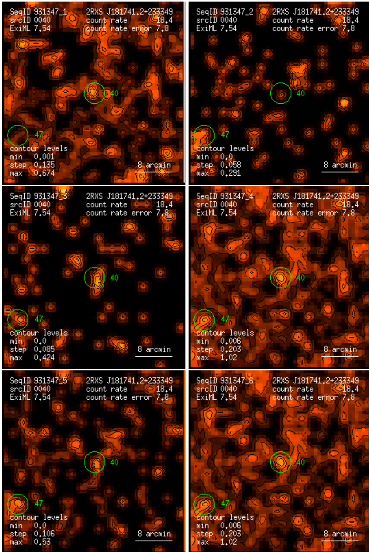
Figure 40: RASS 931347: detection 0040: band rate images, Gaussian filter: (1) PSPC channels 11 – 41, (2) 52 – 90, (3) 91 – 201, (4) 11 – 235, (5) 52 – 201, (6) 11 – 201. Broad band rates in counts/ks. Band rate contour levels in counts/ks/arcmin 2 .
