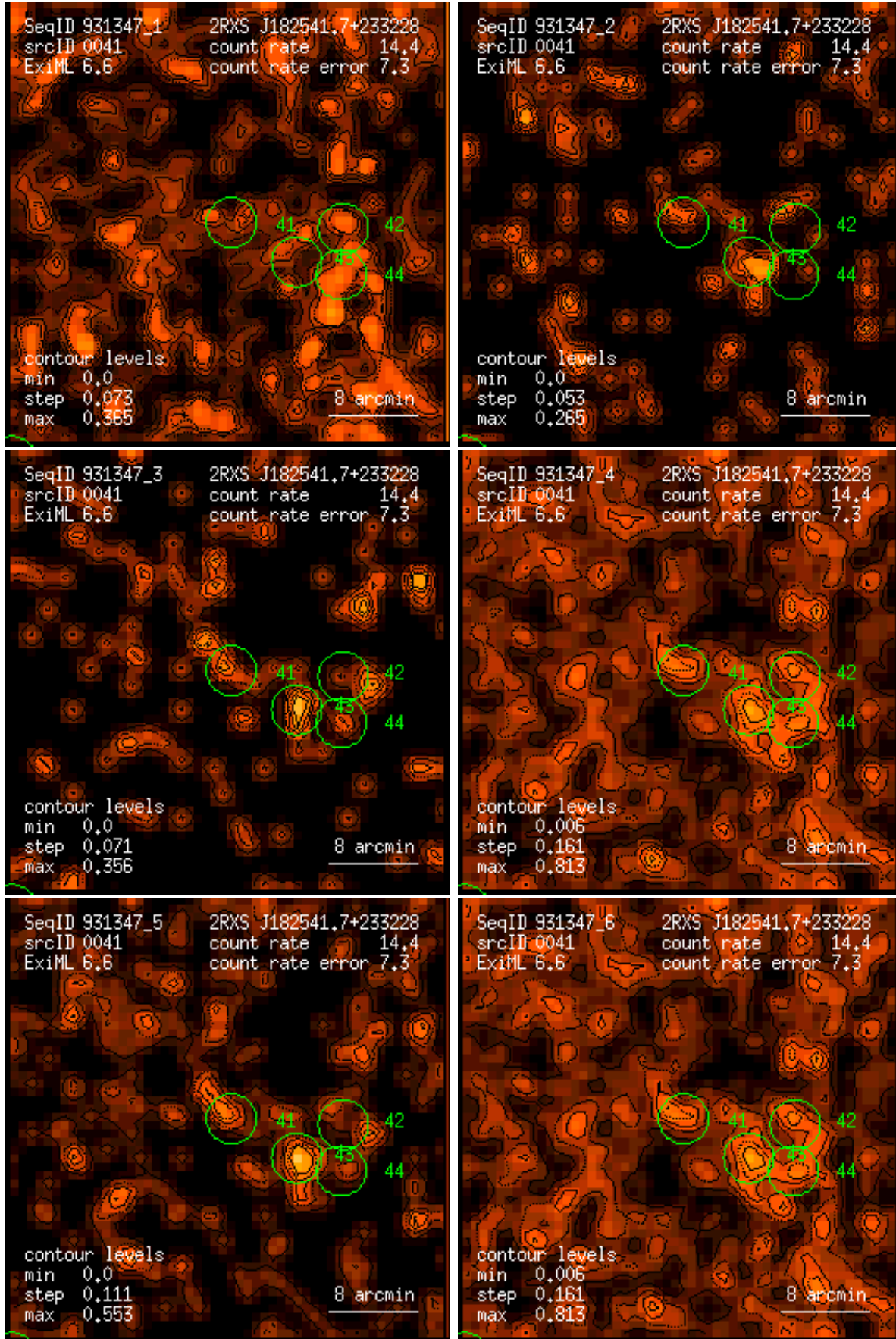
Figure 41: RASS 931347: detection 0041: band rate images, Gaussian filter: (1) PSPC channels 11 – 41, (2) 52 – 90, (3) 91 – 201, (4) 11 – 235, (5) 52 – 201, (6) 11 – 201. Broad band rates in counts/ks. Band rate contour levels in counts/ks/arcmin 2 .
