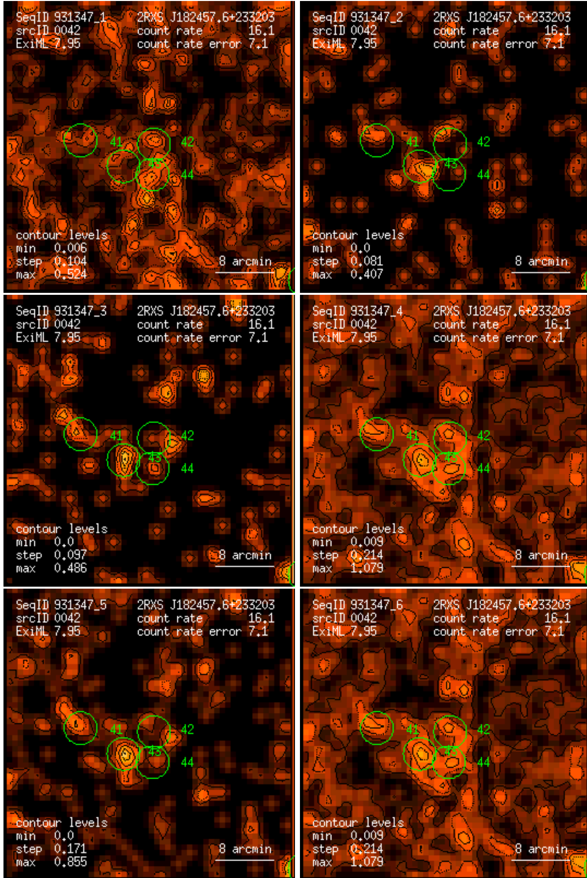
Figure 42: RASS 931347: detection 0042: band rate images, Gaussian filter: (1) PSPC channels 11 – 41, (2) 52 – 90, (3) 91 – 201, (4) 11 – 235, (5) 52 – 201, (6) 11 – 201. Broad band rates in counts/ks. Band rate contour levels in counts/ks/arcmin 2 .
