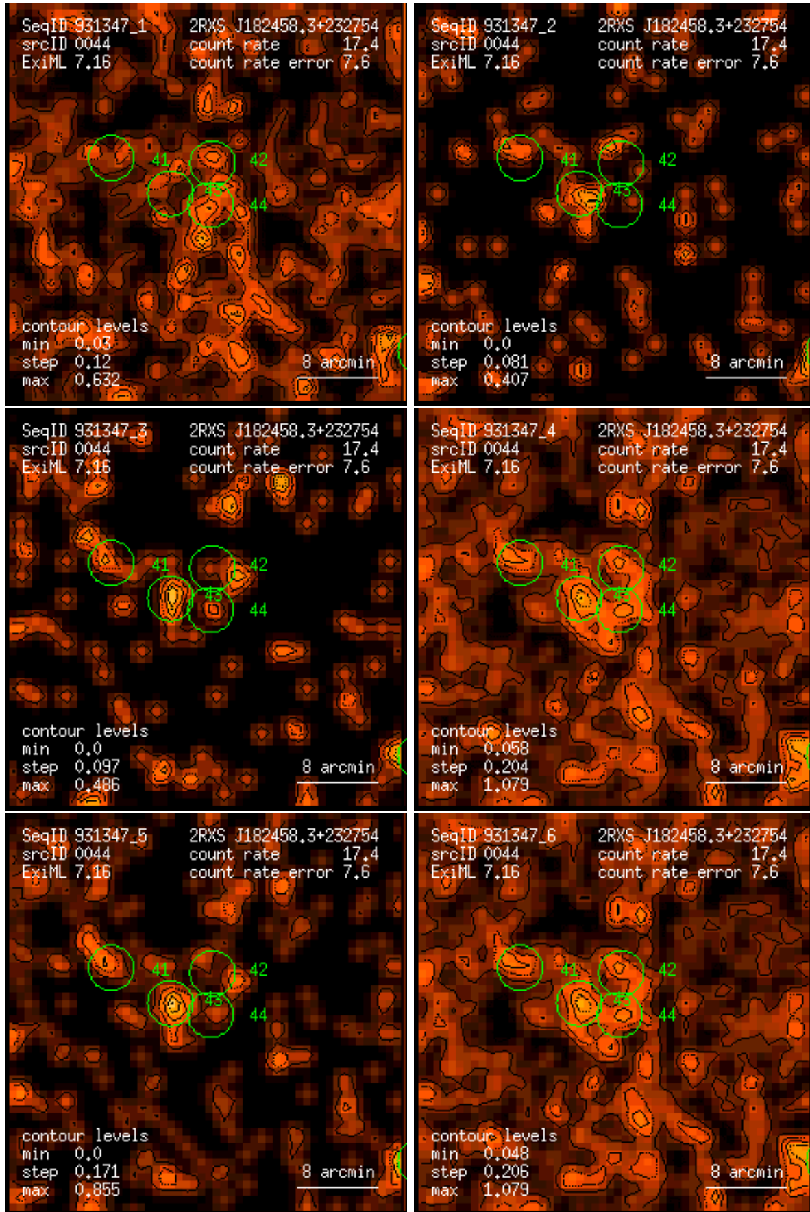
Figure 44: RASS 931347: detection 0044: band rate images, Gaussian filter: (1) PSPC channels 11 – 41, (2) 52 – 90, (3) 91 – 201, (4) 11 – 235, (5) 52 – 201, (6) 11 – 201. Broad band rates in counts/ks. Band rate contour levels in counts/ks/arcmin 2 .
