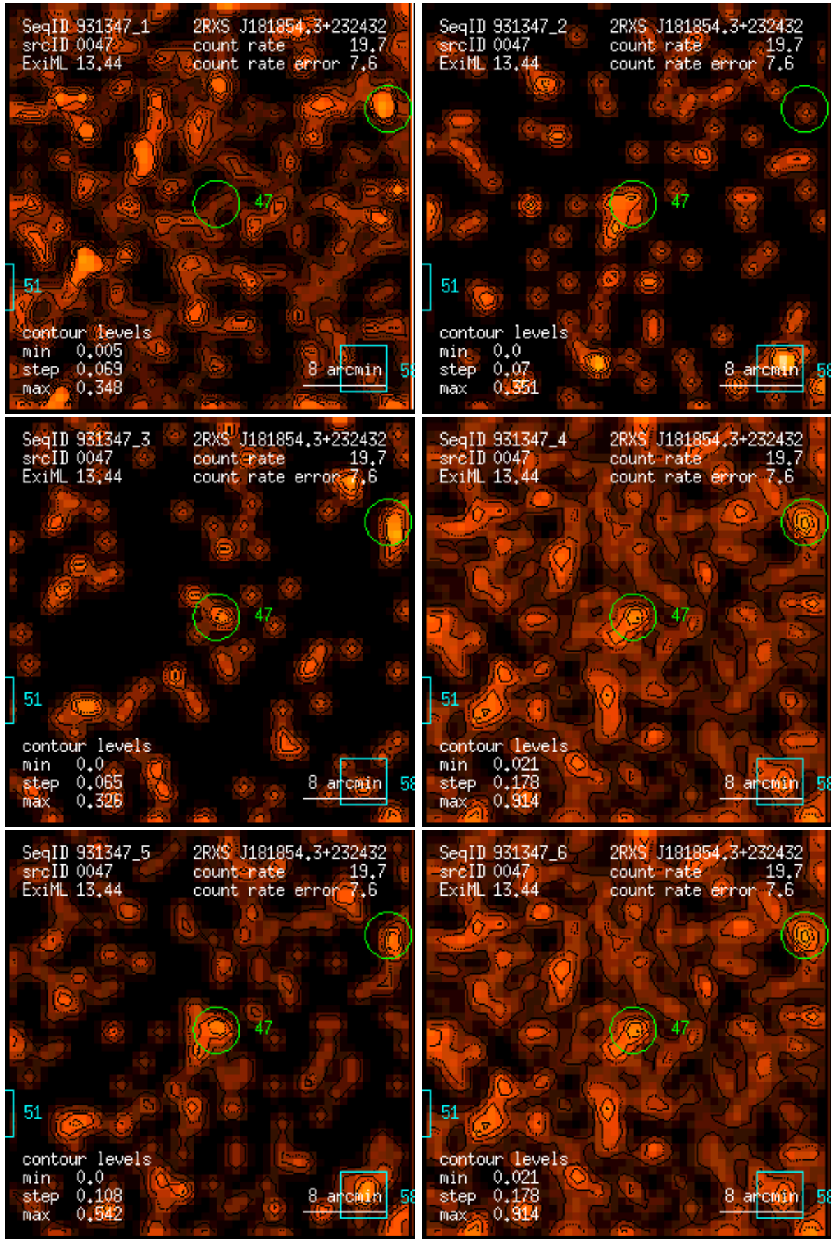
Figure 47: RASS 931347: detection 0047: band rate images, Gaussian filter: (1) PSPC channels 11 – 41, (2) 52 – 90, (3) 91 – 201, (4) 11 – 235, (5) 52 – 201, (6) 11 – 201. Broad band rates in counts/ks. Band rate contour levels in counts/ks/arcmin 2 .
