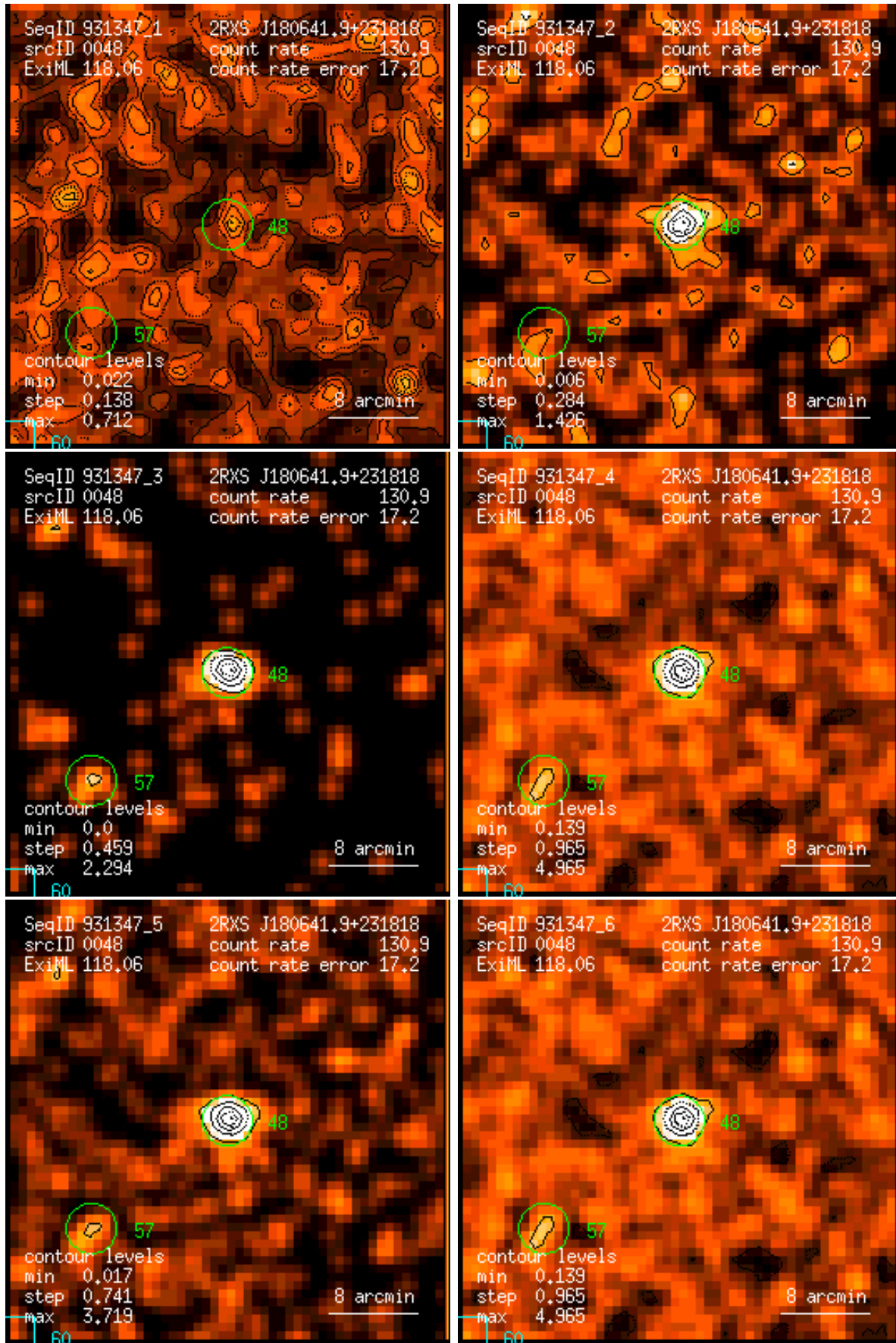
Figure 48: RASS 931347: detection 0048: band rate images, Gaussian filter: (1) PSPC channels 11 – 41, (2) 52 – 90, (3) 91 – 201, (4) 11 – 235, (5) 52 – 201, (6) 11 – 201. Broad band rates in counts/ks. Band rate contour levels in counts/ks/arcmin 2 .
