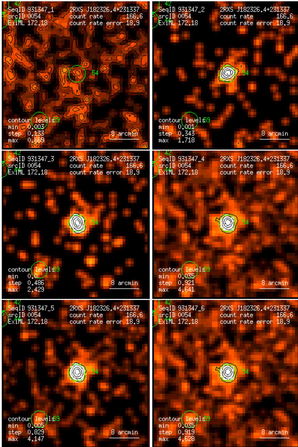
Figure 54: RASS 931347: detection 0054: band rate images, Gaussian filter: (1) PSPC channels 11 – 41, (2) 52 – 90, (3) 91 – 201, (4) 11 – 235, (5) 52 – 201, (6) 11 – 201. Broad band rates in counts/ks. Band rate contour levels in counts/ks/arcmin 2 .
