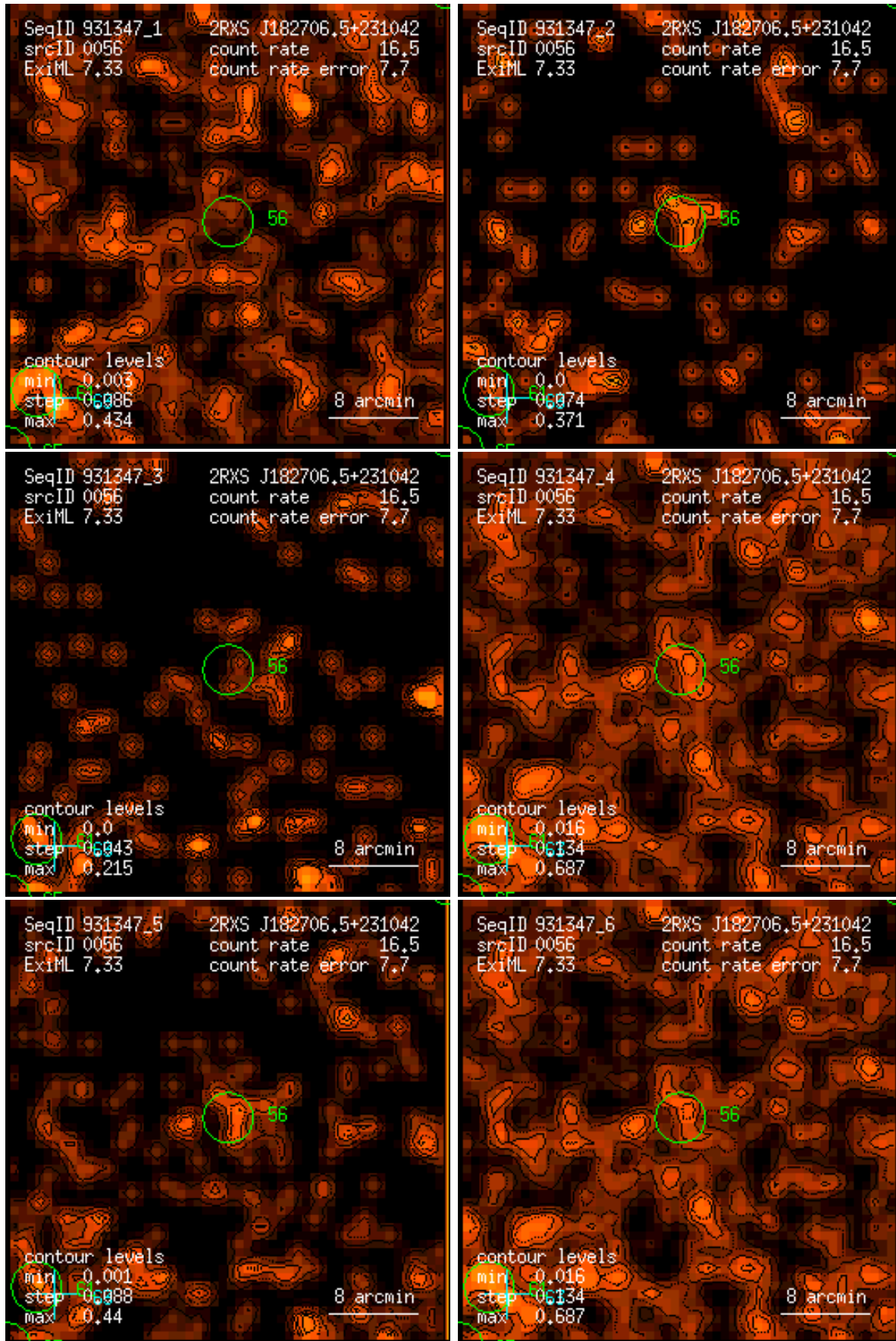
Figure 56: RASS 931347: detection 0056: band rate images, Gaussian filter: (1) PSPC channels 11 – 41, (2) 52 – 90, (3) 91 – 201, (4) 11 – 235, (5) 52 – 201, (6) 11 – 201. Broad band rates in counts/ks. Band rate contour levels in counts/ks/arcmin 2 .
