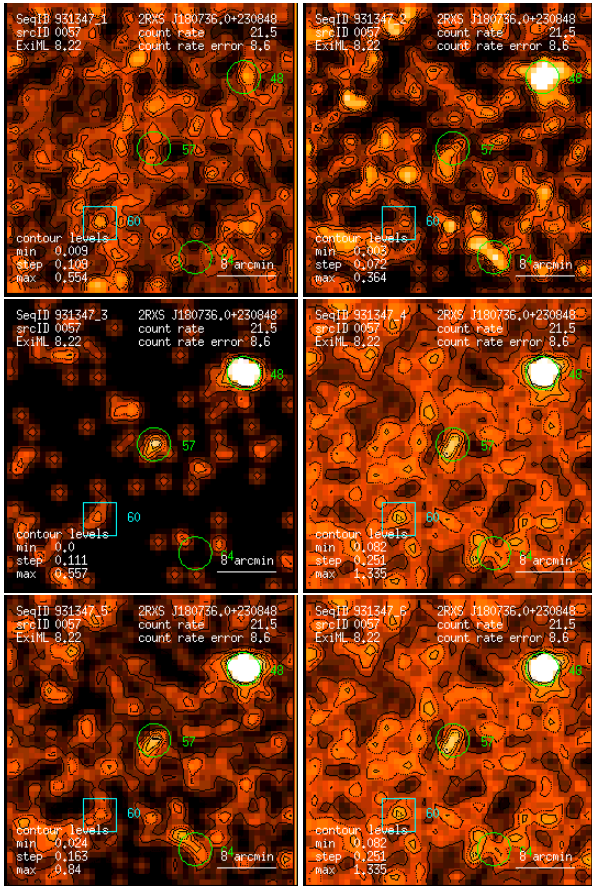
Figure 57: RASS 931347: detection 0057: band rate images, Gaussian filter: (1) PSPC channels 11 – 41, (2) 52 – 90, (3) 91 – 201, (4) 11 – 235, (5) 52 – 201, (6) 11 – 201. Broad band rates in counts/ks. Band rate contour levels in counts/ks/arcmin 2 .
