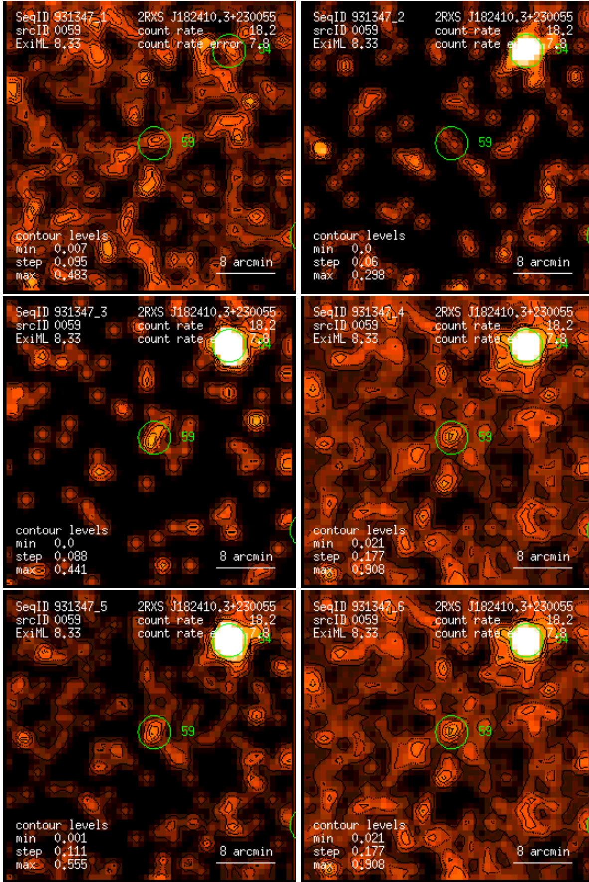
Figure 59: RASS 931347: detection 0059: band rate images, Gaussian filter: (1) PSPC channels 11 – 41, (2) 52 – 90, (3) 91 – 201, (4) 11 – 235, (5) 52 – 201, (6) 11 – 201. Broad band rates in counts/ks. Band rate contour levels in counts/ks/arcmin 2 .
