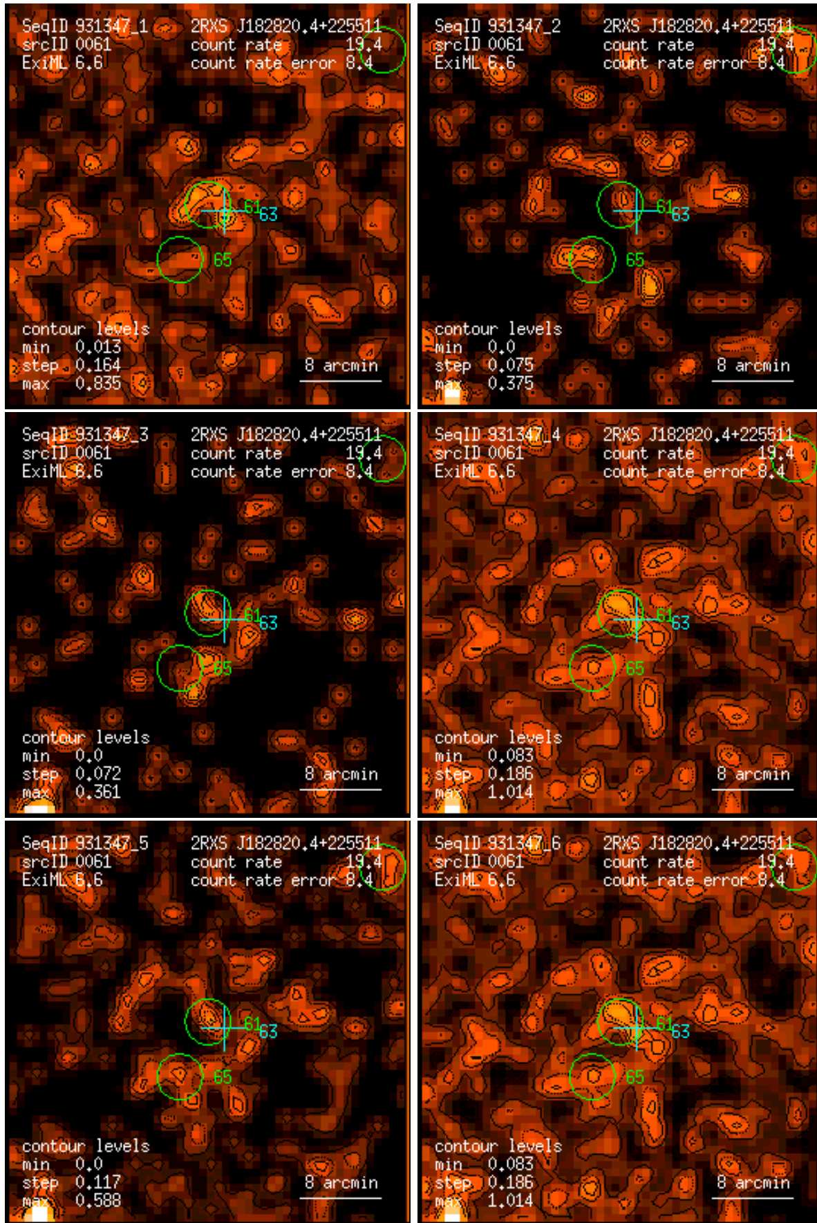
Figure 61: RASS 931347: detection 0061: band rate images, Gaussian filter: (1) PSPC channels 11 – 41, (2) 52 – 90, (3) 91 – 201, (4) 11 – 235, (5) 52 – 201, (6) 11 – 201. Broad band rates in counts/ks. Band rate contour levels in counts/ks/arcmin 2 .
