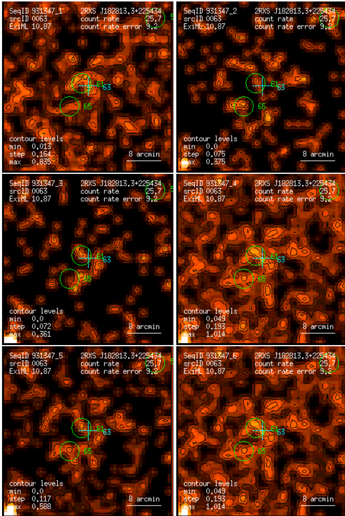
Figure 63: RASS 931347: detection 0063: band rate images, Gaussian filter: (1) PSPC channels 11 – 41, (2) 52 – 90, (3) 91 – 201, (4) 11 – 235, (5) 52 – 201, (6) 11 – 201. Broad band rates in counts/ks. Band rate contour levels in counts/ks/arcmin 2 .
