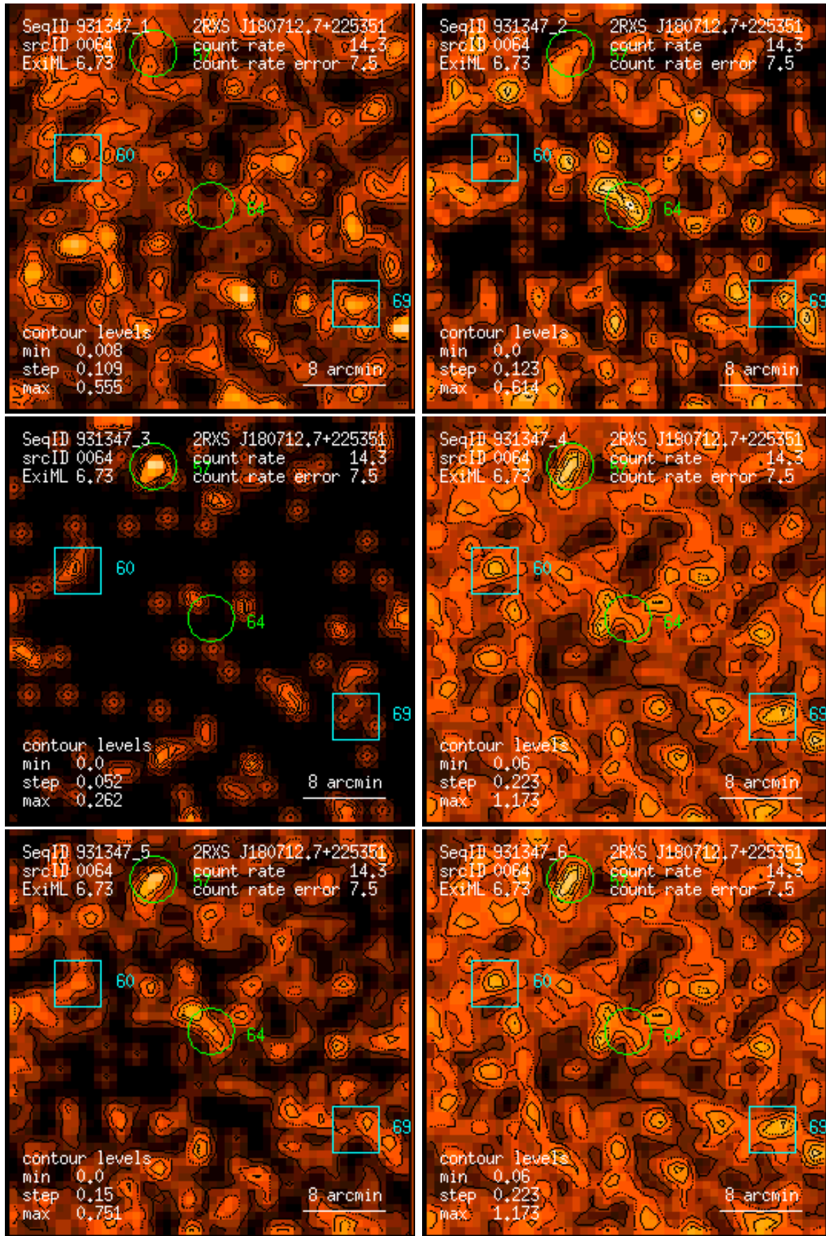
Figure 64: RASS 931347: detection 0064: band rate images, Gaussian filter: (1) PSPC channels 11 – 41, (2) 52 – 90, (3) 91 – 201, (4) 11 – 235, (5) 52 – 201, (6) 11 – 201. Broad band rates in counts/ks. Band rate contour levels in counts/ks/arcmin 2 .
