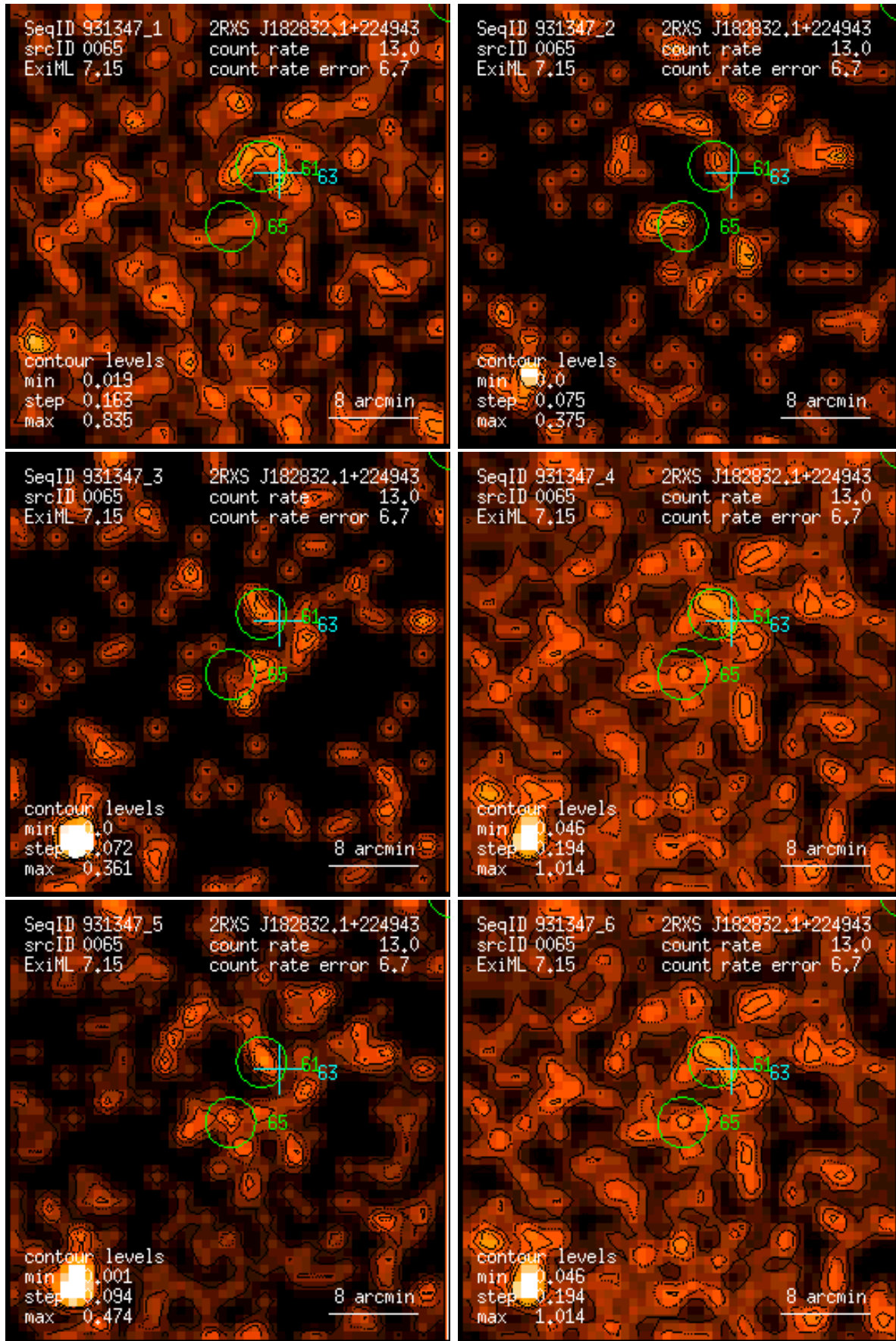
Figure 65: RASS 931347: detection 0065: band rate images, Gaussian filter: (1) PSPC channels 11 – 41, (2) 52 – 90, (3) 91 – 201, (4) 11 – 235, (5) 52 – 201, (6) 11 – 201. Broad band rates in counts/ks. Band rate contour levels in counts/ks/arcmin 2 .
