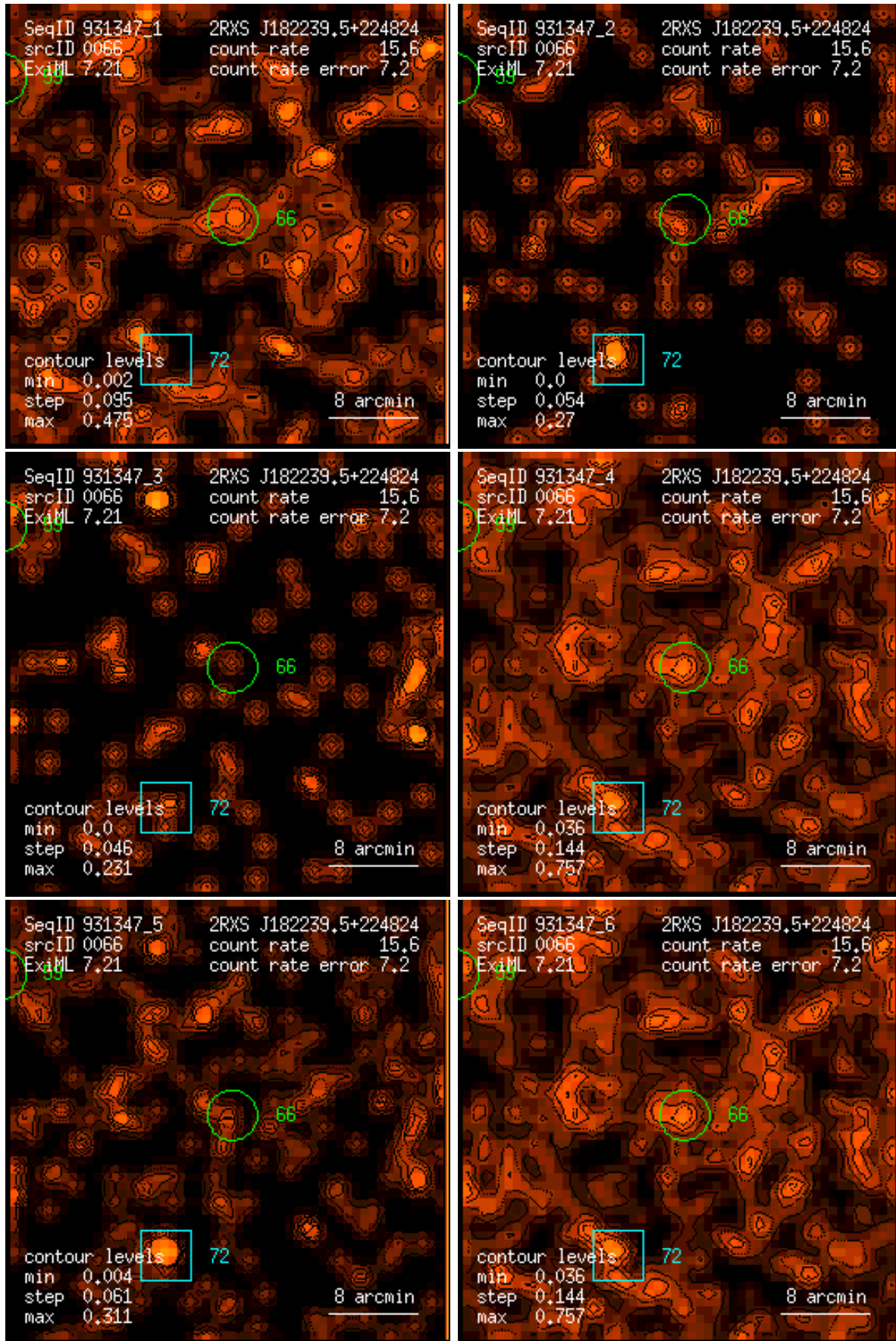
Figure 66: RASS 931347: detection 0066: band rate images, Gaussian filter: (1) PSPC channels 11 – 41, (2) 52 – 90, (3) 91 – 201, (4) 11 – 235, (5) 52 – 201, (6) 11 – 201. Broad band rates in counts/ks. Band rate contour levels in counts/ks/arcmin 2 .
