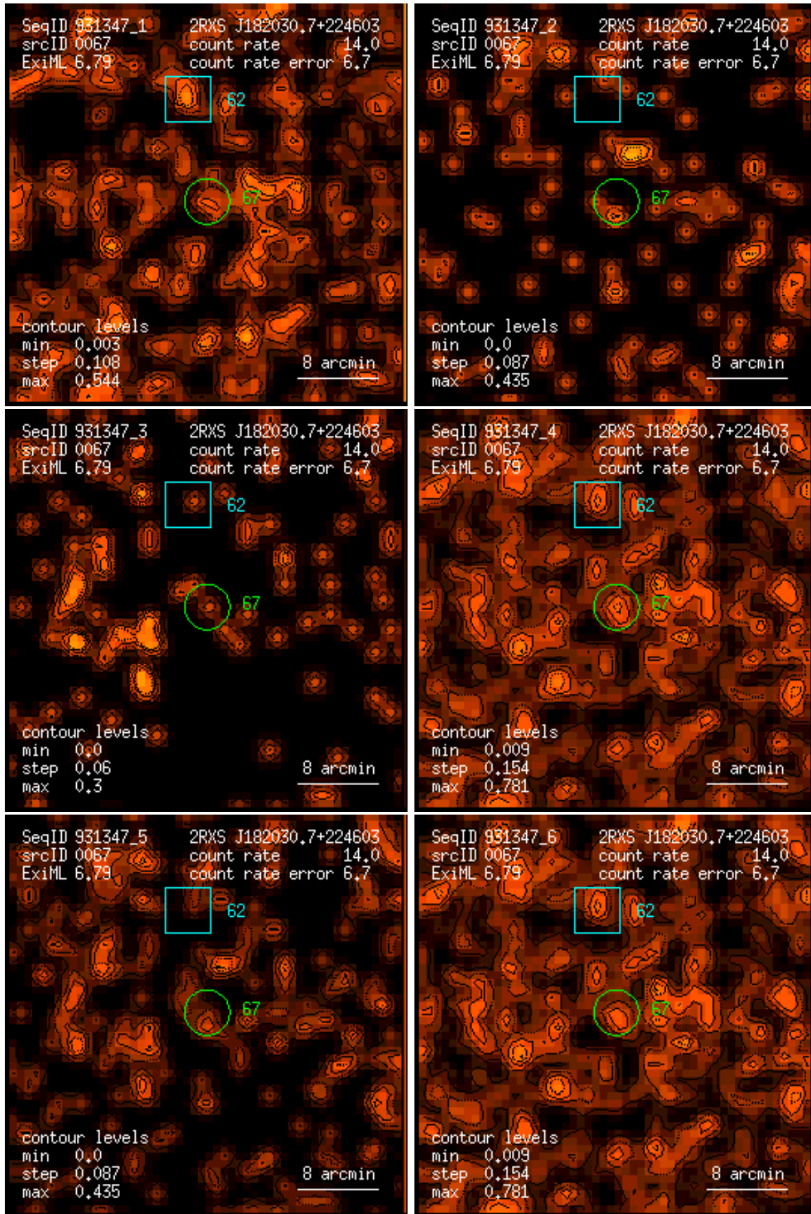
Figure 67: RASS 931347: detection 0067: band rate images, Gaussian filter: (1) PSPC channels 11 – 41, (2) 52 – 90, (3) 91 – 201, (4) 11 – 235, (5) 52 – 201, (6) 11 – 201. Broad band rates in counts/ks. Band rate contour levels in counts/ks/arcmin 2 .
