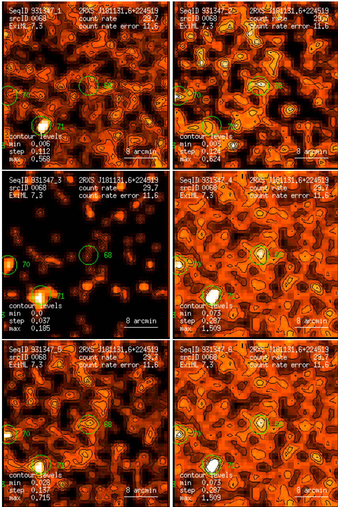
Figure 68: RASS 931347: detection 0068: band rate images, Gaussian filter: (1) PSPC channels 11 – 41, (2) 52 – 90, (3) 91 – 201, (4) 11 – 235, (5) 52 – 201, (6) 11 – 201. Broad band rates in counts/ks. Band rate contour levels in counts/ks/arcmin 2 .
