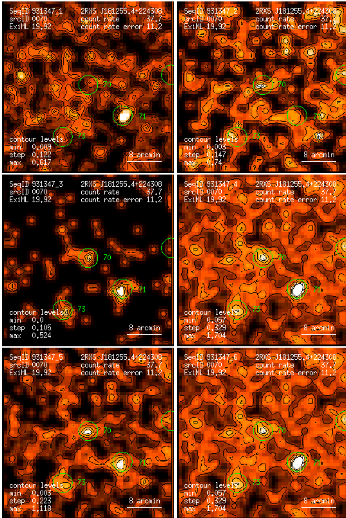
Figure 70: RASS 931347: detection 0070: band rate images, Gaussian filter: (1) PSPC channels 11 – 41, (2) 52 – 90, (3) 91 – 201, (4) 11 – 235, (5) 52 – 201, (6) 11 – 201. Broad band rates in counts/ks. Band rate contour levels in counts/ks/arcmin 2 .
