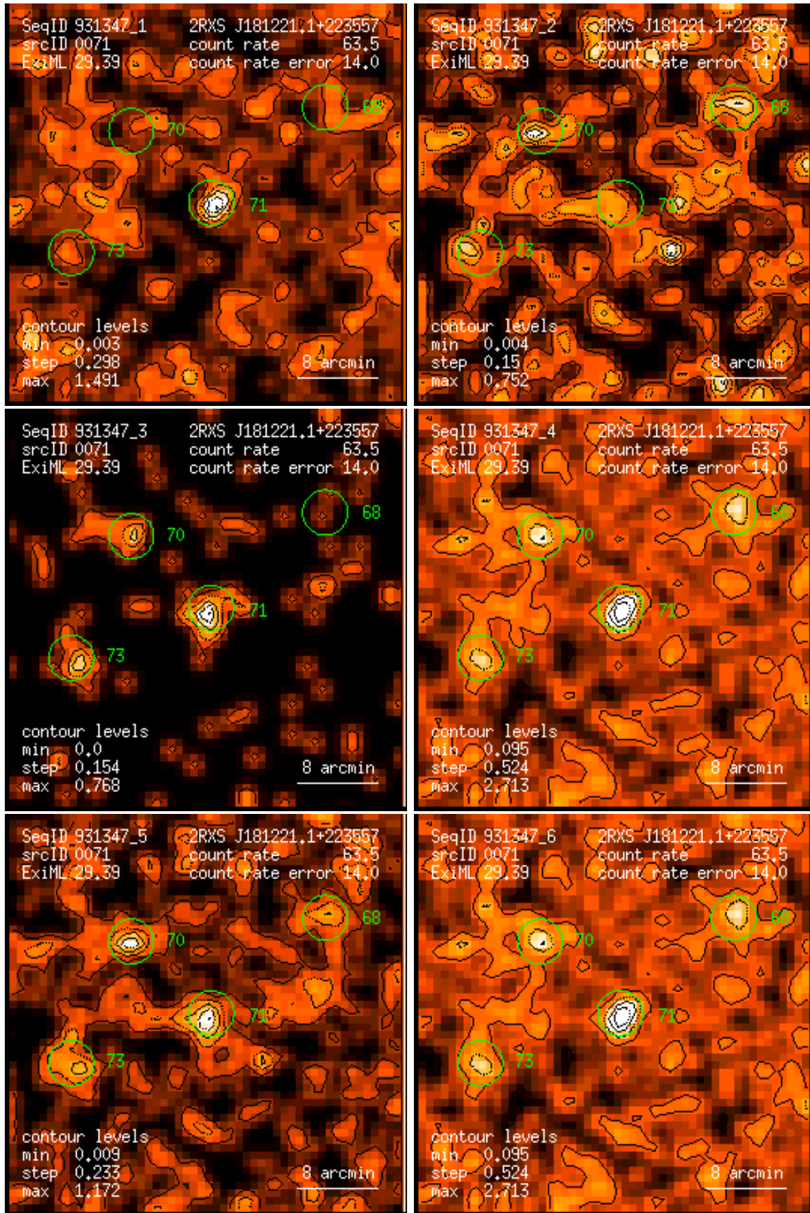
Figure 71: RASS 931347: detection 0071: band rate images, Gaussian filter: (1) PSPC channels 11 – 41, (2) 52 – 90, (3) 91 – 201, (4) 11 – 235, (5) 52 – 201, (6) 11 – 201. Broad band rates in counts/ks. Band rate contour levels in counts/ks/arcmin 2 .
