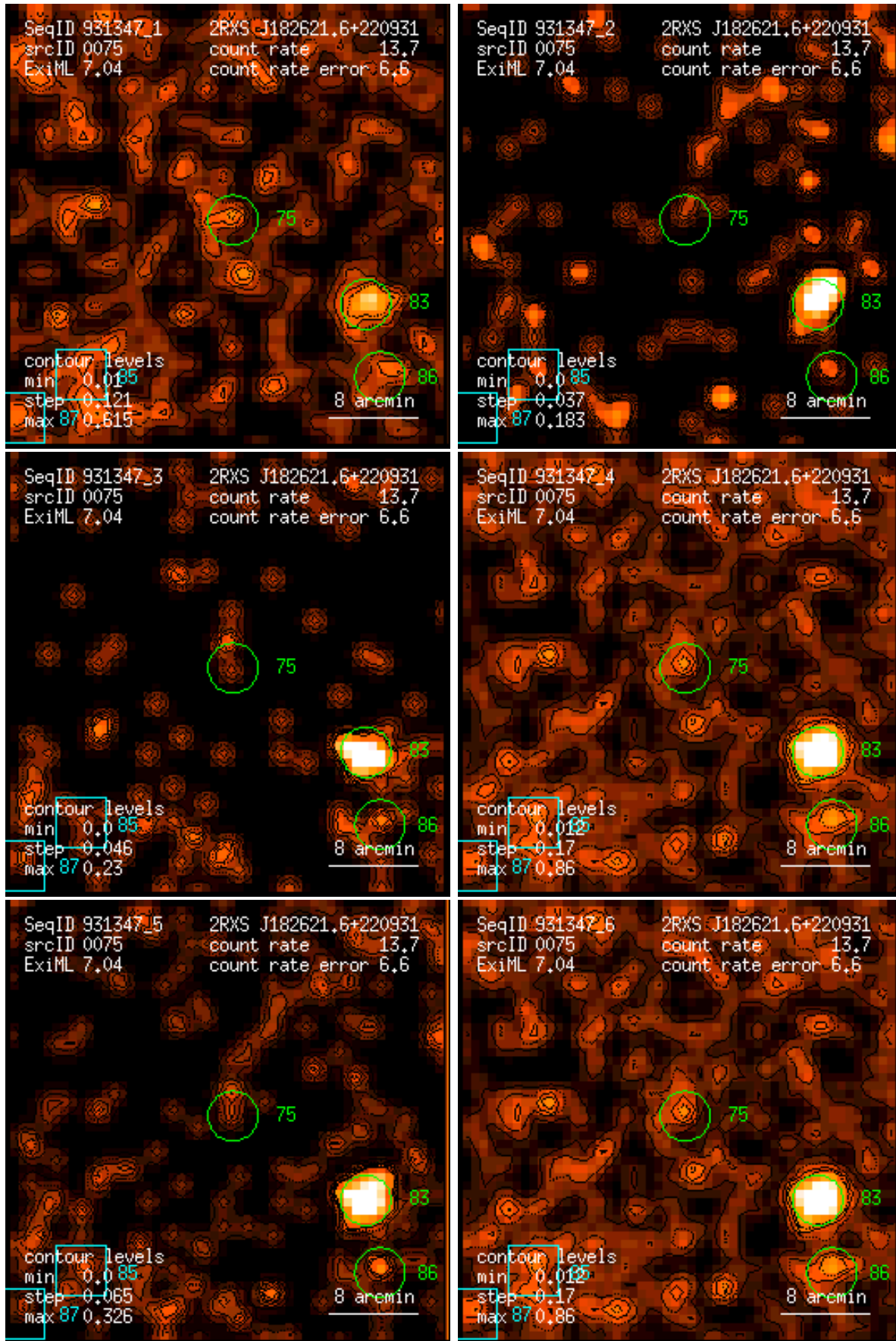
Figure 75: RASS 931347: detection 0075: band rate images, Gaussian filter: (1) PSPC channels 11 – 41, (2) 52 – 90, (3) 91 – 201, (4) 11 – 235, (5) 52 – 201, (6) 11 – 201. Broad band rates in counts/ks. Band rate contour levels in counts/ks/arcmin 2 .
