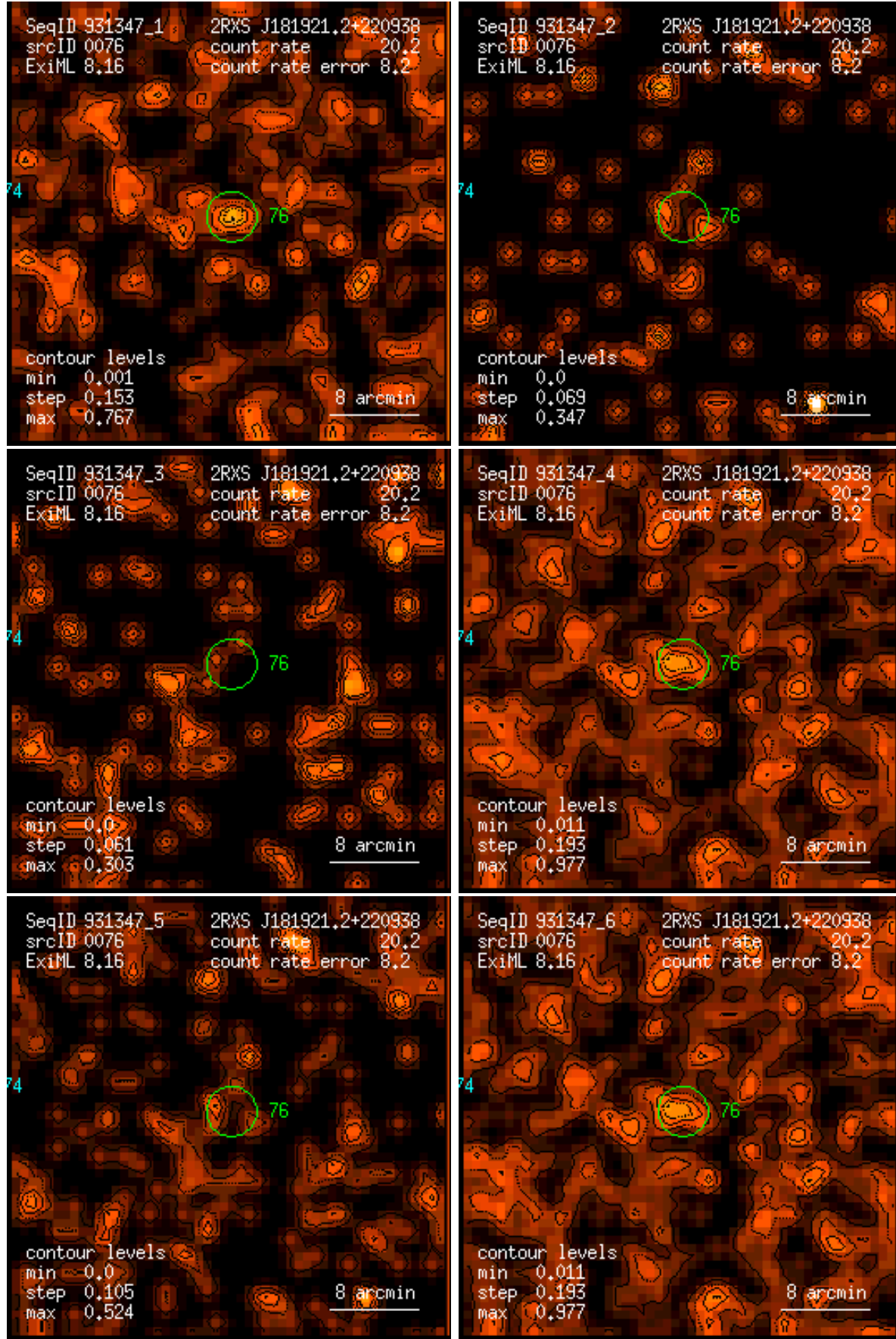
Figure 76: RASS 931347: detection 0076: band rate images, Gaussian filter: (1) PSPC channels 11 – 41, (2) 52 – 90, (3) 91 – 201, (4) 11 – 235, (5) 52 – 201, (6) 11 – 201. Broad band rates in counts/ks. Band rate contour levels in counts/ks/arcmin 2 .
