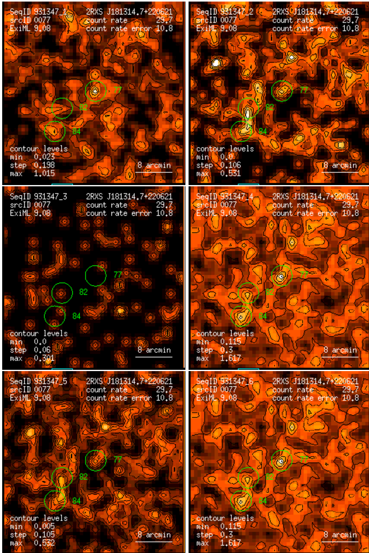
Figure 77: RASS 931347: detection 0077: band rate images, Gaussian filter: (1) PSPC channels 11 – 41, (2) 52 – 90, (3) 91 – 201, (4) 11 – 235, (5) 52 – 201, (6) 11 – 201. Broad band rates in counts/ks. Band rate contour levels in counts/ks/arcmin 2 .
