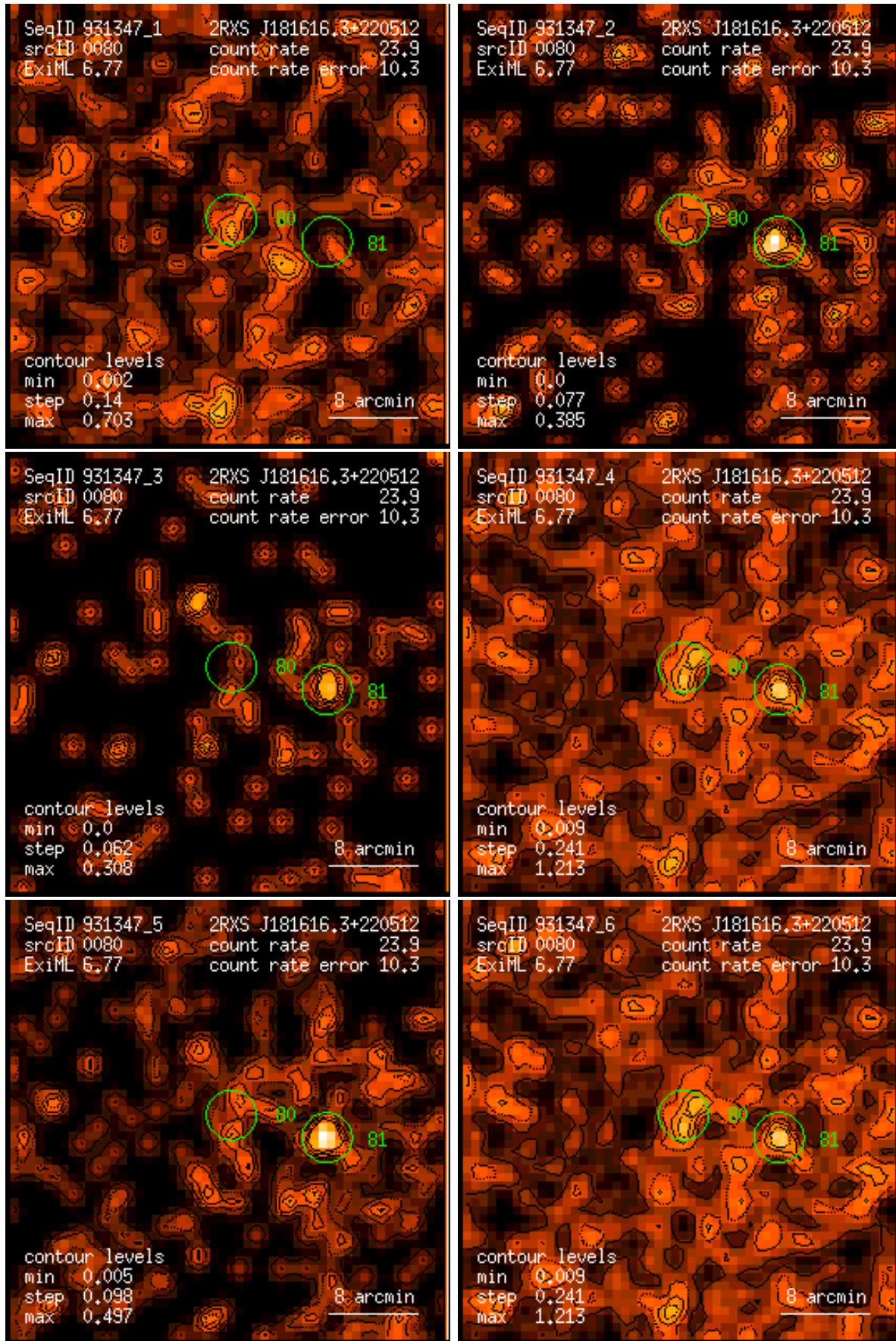
Figure 80: RASS 931347: detection 0080: band rate images, Gaussian filter: (1) PSPC channels 11 – 41, (2) 52 – 90, (3) 91 – 201, (4) 11 – 235, (5) 52 – 201, (6) 11 – 201. Broad band rates in counts/ks. Band rate contour levels in counts/ks/arcmin 2 .
