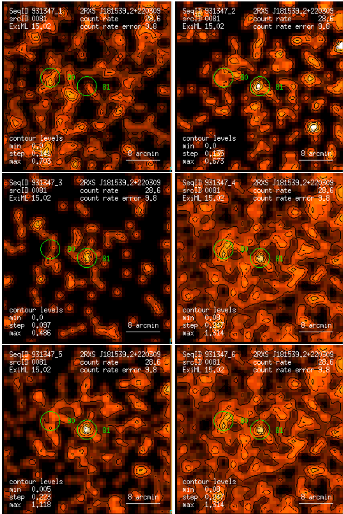
Figure 81: RASS 931347: detection 0081: band rate images, Gaussian filter: (1) PSPC channels 11 – 41, (2) 52 – 90, (3) 91 – 201, (4) 11 – 235, (5) 52 – 201, (6) 11 – 201. Broad band rates in counts/ks. Band rate contour levels in counts/ks/arcmin 2 .
