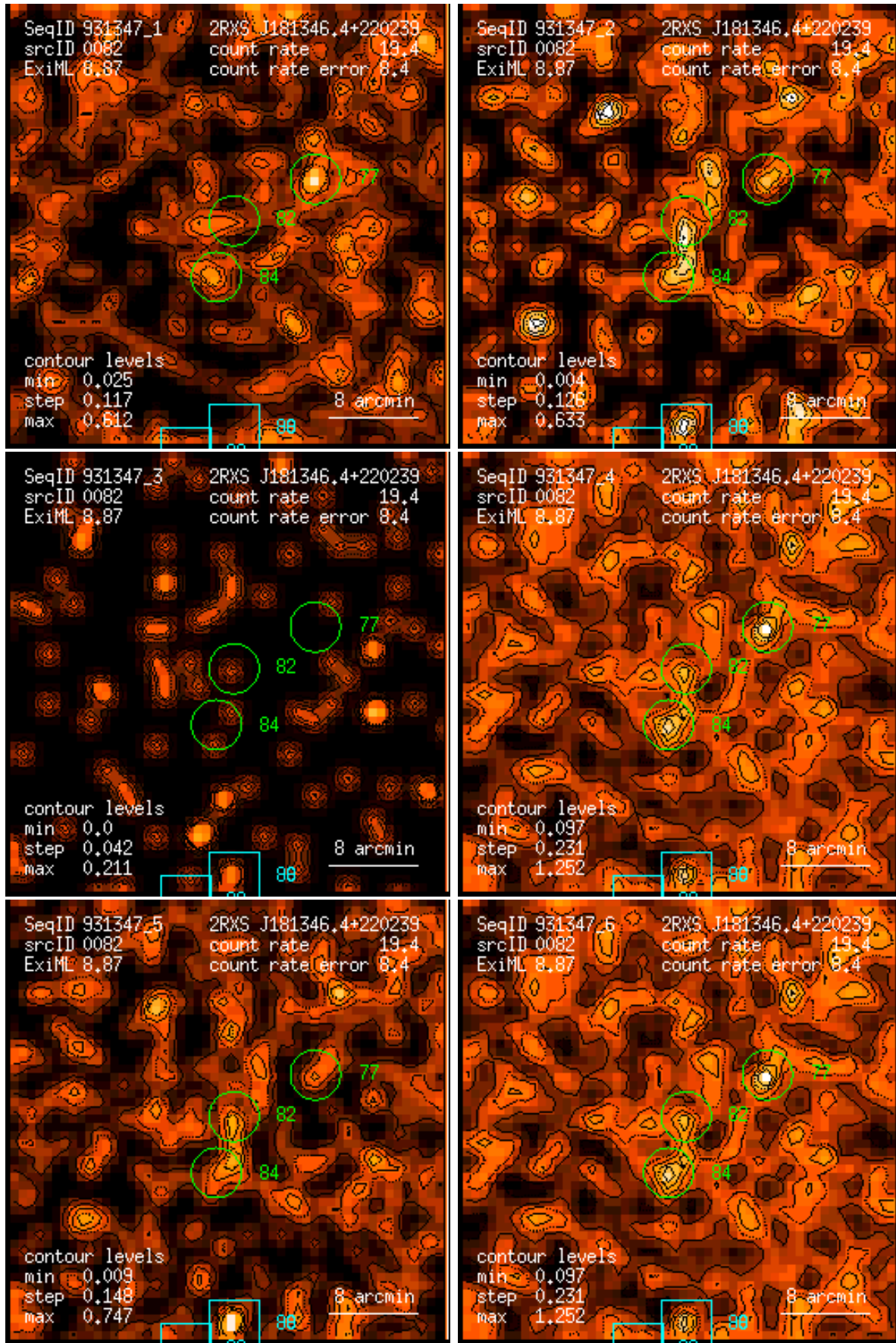
Figure 82: RASS 931347: detection 0082: band rate images, Gaussian filter: (1) PSPC channels 11 – 41, (2) 52 – 90, (3) 91 – 201, (4) 11 – 235, (5) 52 – 201, (6) 11 – 201. Broad band rates in counts/ks. Band rate contour levels in counts/ks/arcmin 2 .
