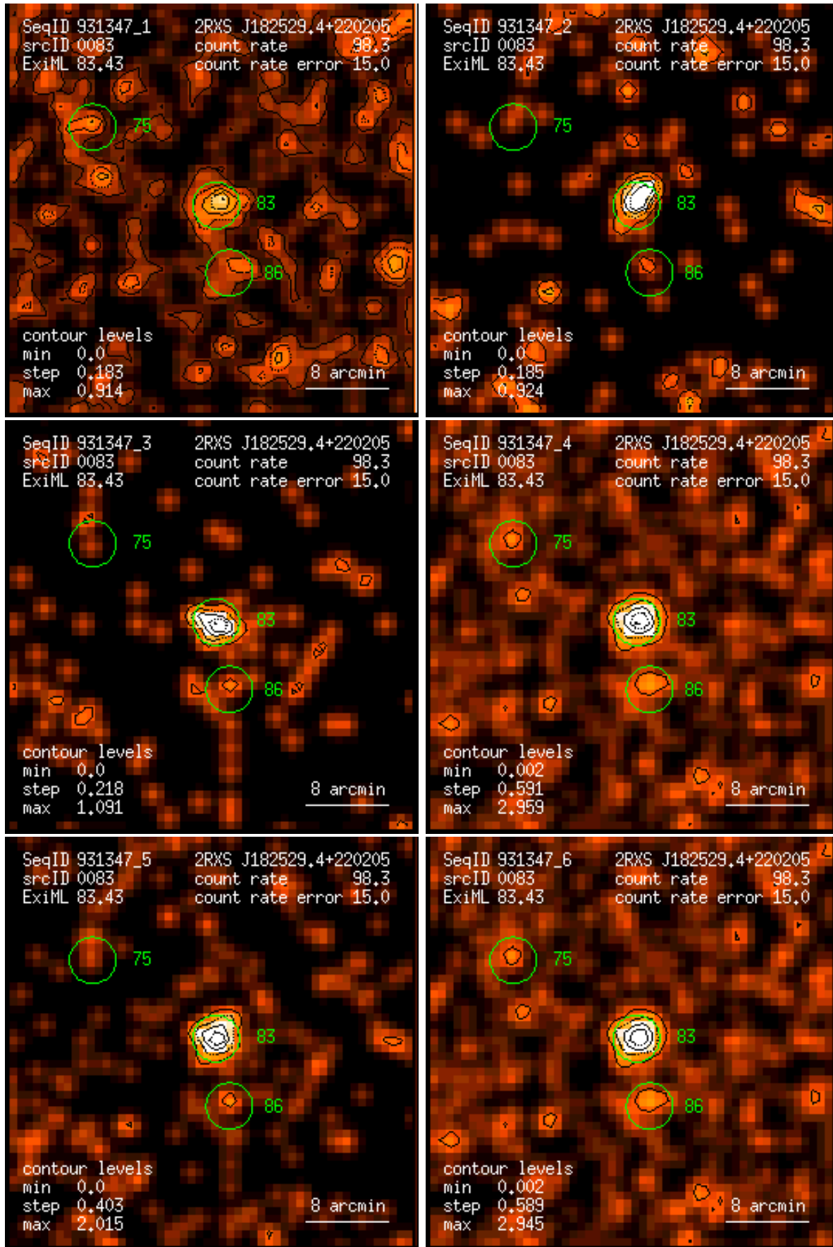
Figure 83: RASS 931347: detection 0083: band rate images, Gaussian filter: (1) PSPC channels 11 – 41, (2) 52 – 90, (3) 91 – 201, (4) 11 – 235, (5) 52 – 201, (6) 11 – 201. Broad band rates in counts/ks. Band rate contour levels in counts/ks/arcmin 2 .
