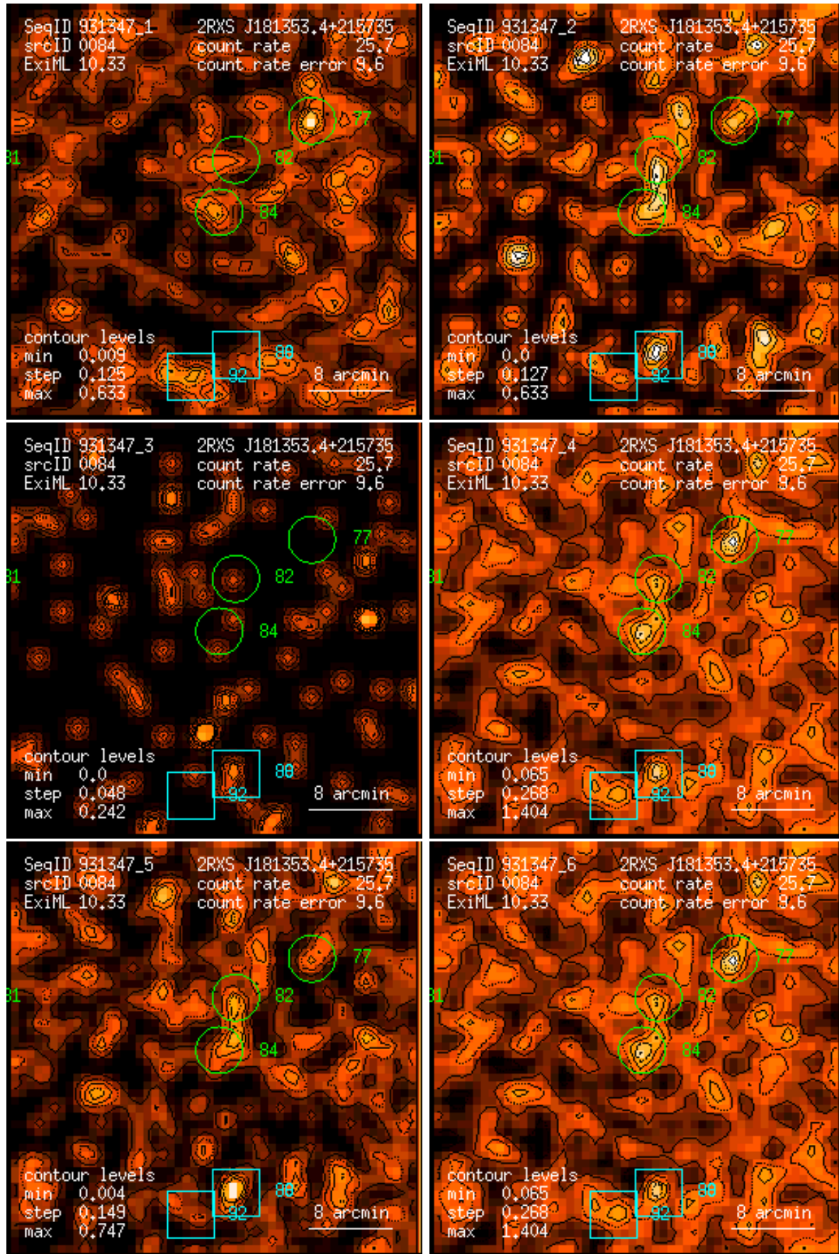
Figure 84: RASS 931347: detection 0084: band rate images, Gaussian filter: (1) PSPC channels 11 – 41, (2) 52 – 90, (3) 91 – 201, (4) 11 – 235, (5) 52 – 201, (6) 11 – 201. Broad band rates in counts/ks. Band rate contour levels in counts/ks/arcmin 2 .
