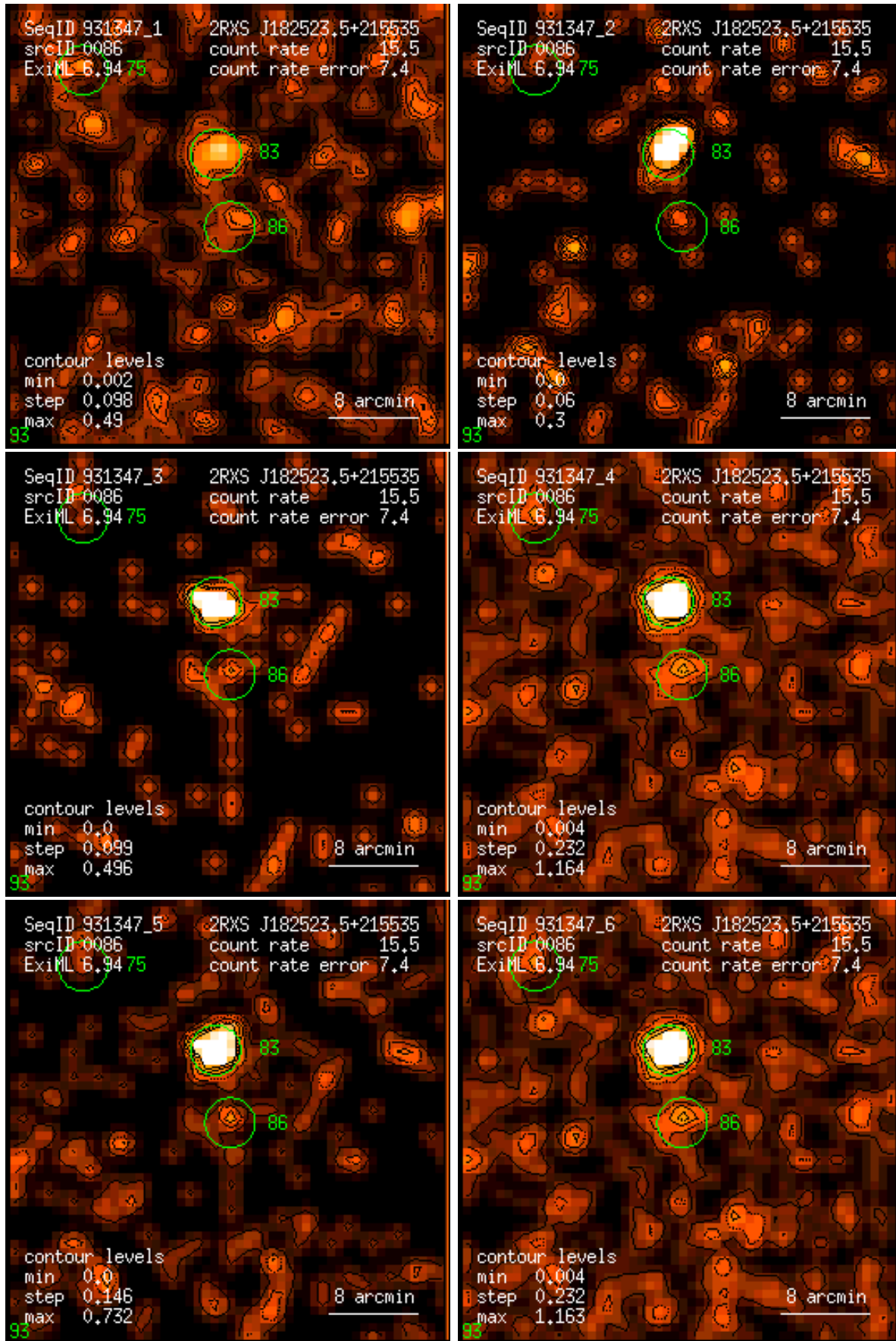
Figure 86: RASS 931347: detection 0086: band rate images, Gaussian filter: (1) PSPC channels 11 – 41, (2) 52 – 90, (3) 91 – 201, (4) 11 – 235, (5) 52 – 201, (6) 11 – 201. Broad band rates in counts/ks. Band rate contour levels in counts/ks/arcmin 2 .
