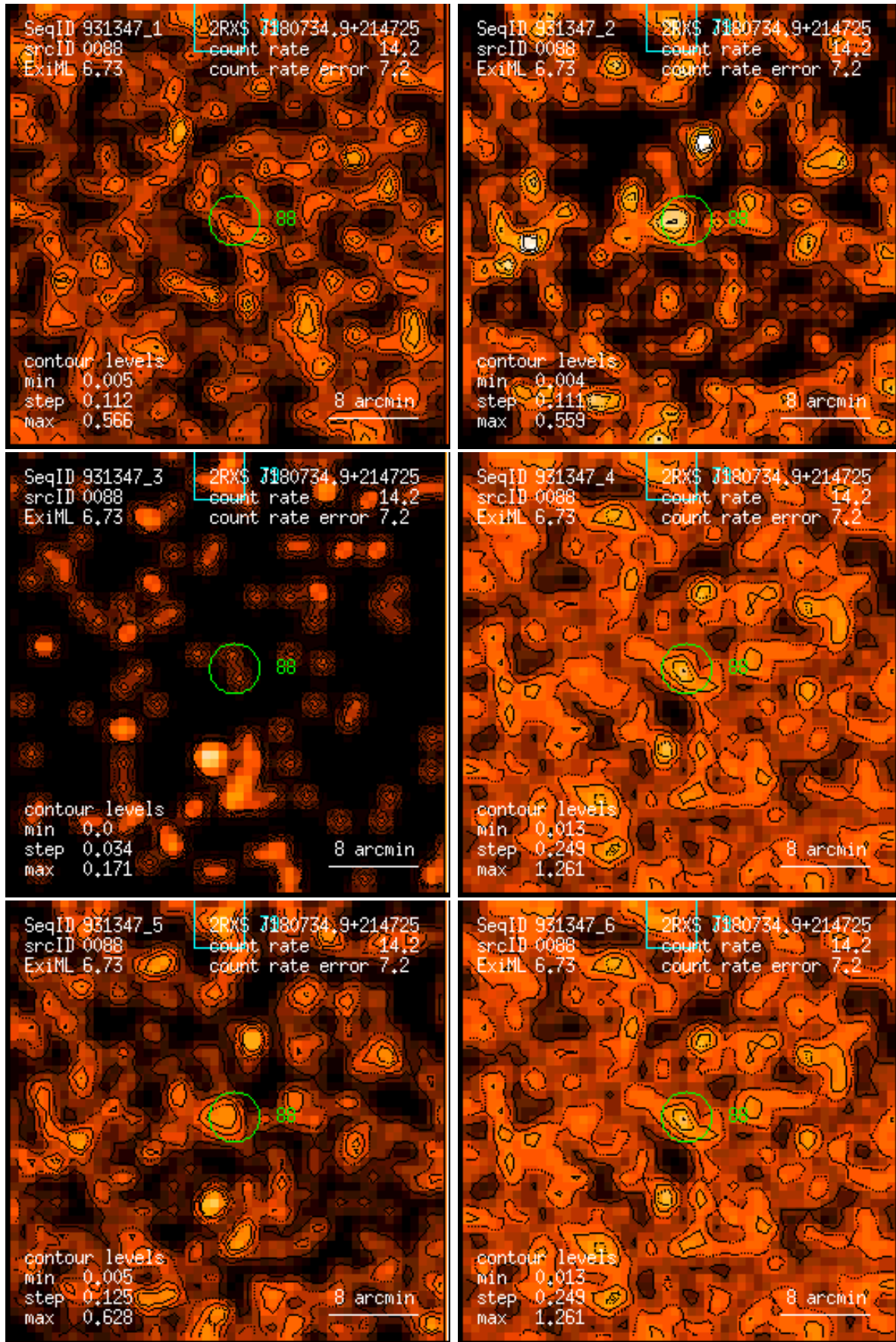
Figure 88: RASS 931347: detection 0088: band rate images, Gaussian filter: (1) PSPC channels 11 – 41, (2) 52 – 90, (3) 91 – 201, (4) 11 – 235, (5) 52 – 201, (6) 11 – 201. Broad band rates in counts/ks. Band rate contour levels in counts/ks/arcmin 2 .
