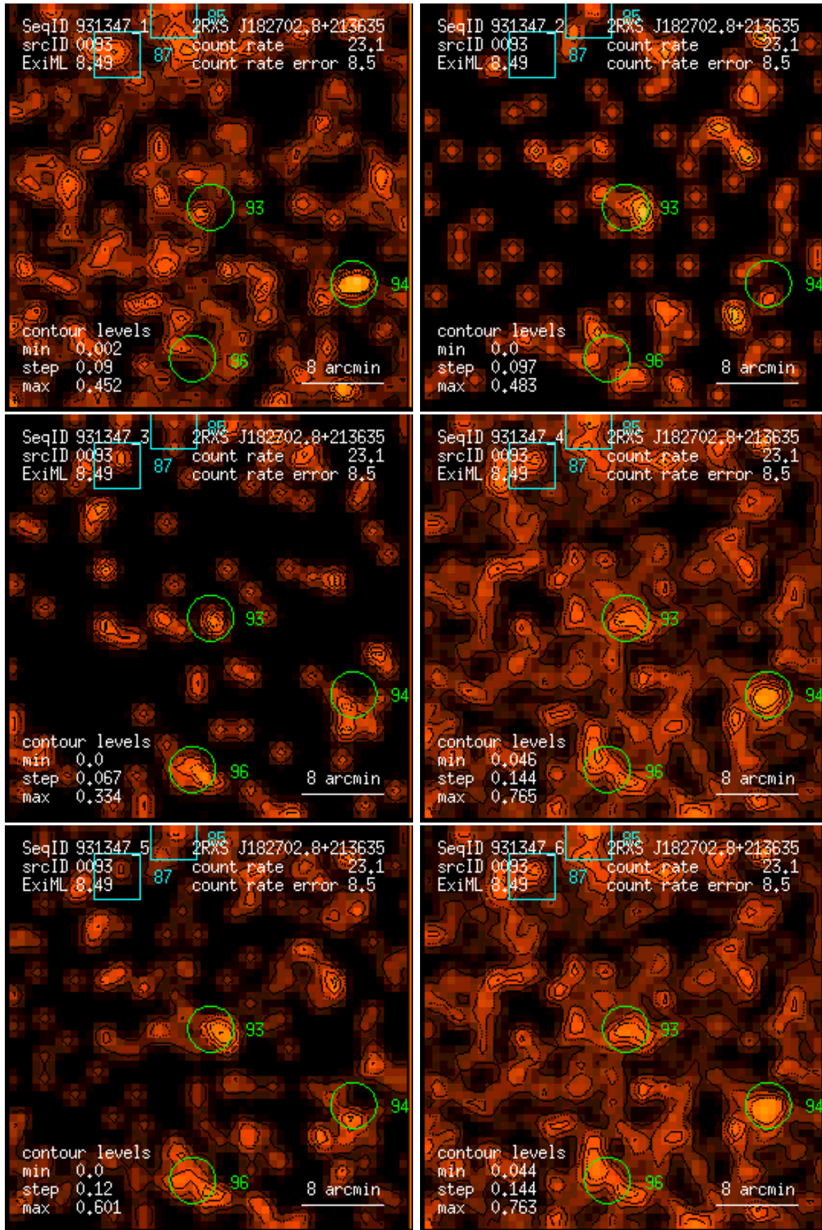
Figure 93: RASS 931347: detection 0093: band rate images, Gaussian filter: (1) PSPC channels 11 – 41, (2) 52 – 90, (3) 91 – 201, (4) 11 – 235, (5) 52 – 201, (6) 11 – 201. Broad band rates in counts/ks. Band rate contour levels in counts/ks/arcmin 2 .
