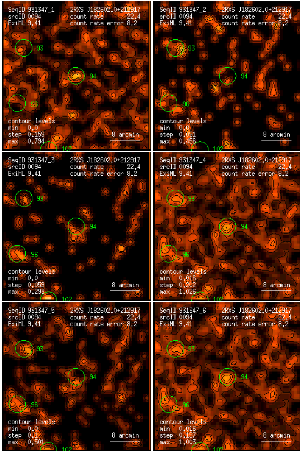
Figure 94: RASS 931347: detection 0094: band rate images, Gaussian filter: (1) PSPC channels 11 – 41, (2) 52 – 90, (3) 91 – 201, (4) 11 – 235, (5) 52 – 201, (6) 11 – 201. Broad band rates in counts/ks. Band rate contour levels in counts/ks/arcmin 2 .
