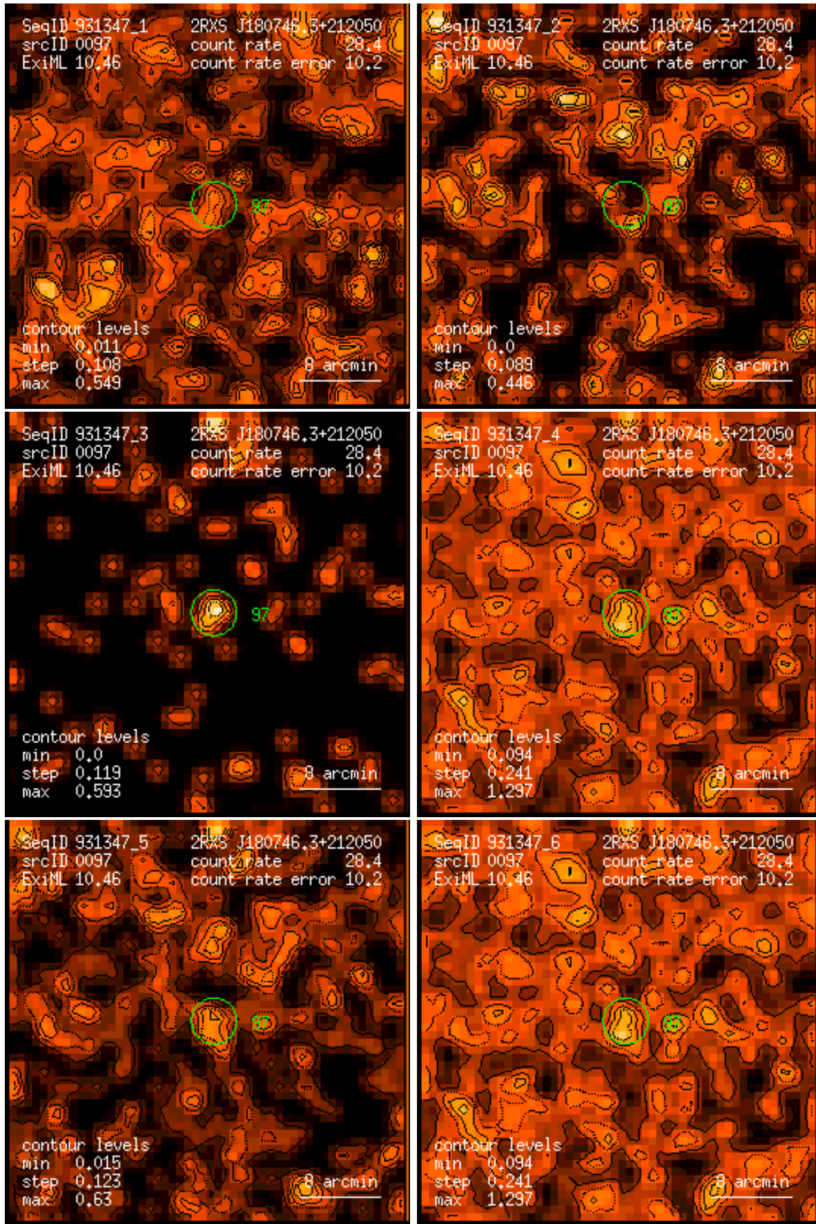
Figure 97: RASS 931347: detection 0097: band rate images, Gaussian filter: (1) PSPC channels 11 – 41, (2) 52 – 90, (3) 91 – 201, (4) 11 – 235, (5) 52 – 201, (6) 11 – 201. Broad band rates in counts/ks. Band rate contour levels in counts/ks/arcmin 2 .
