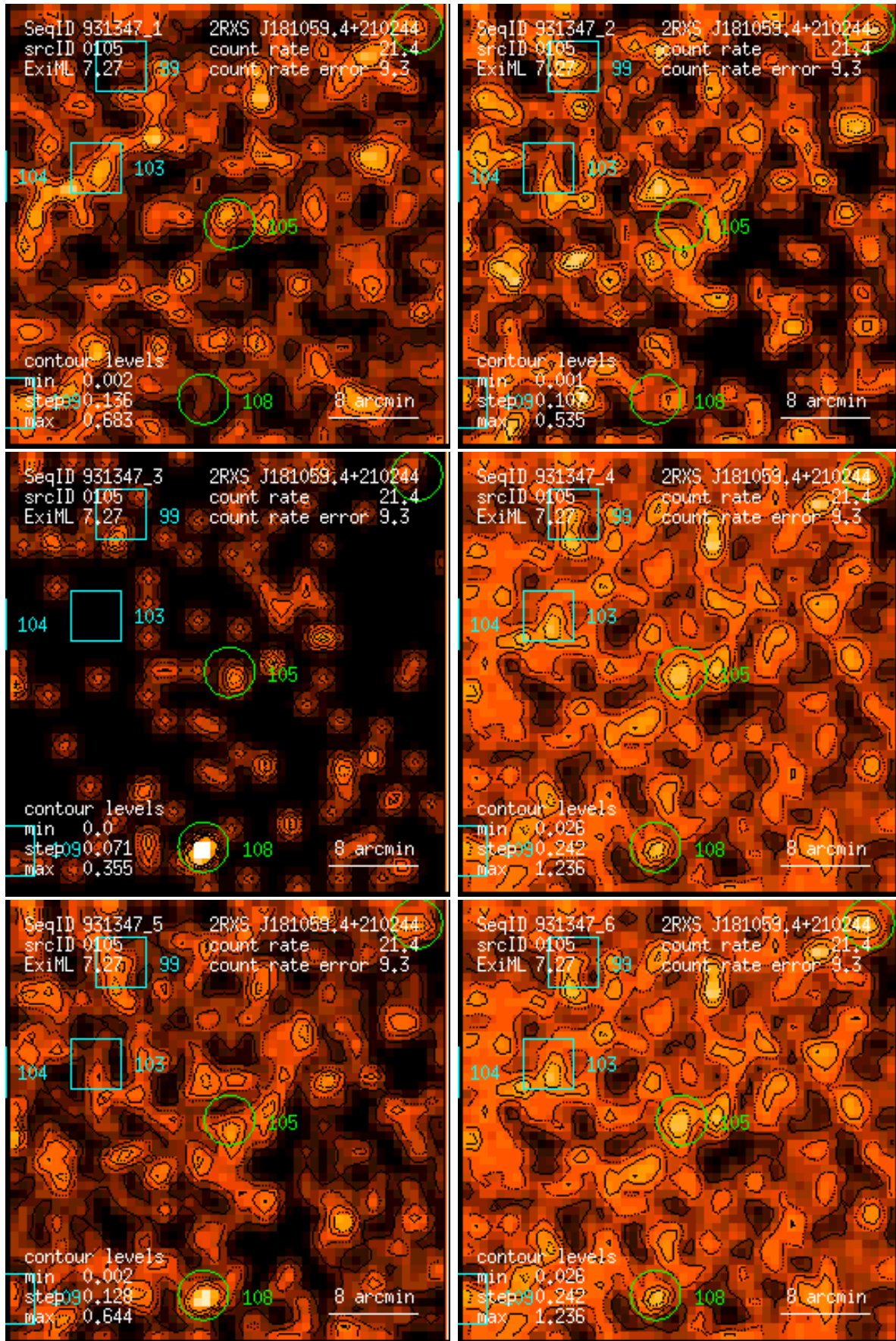
Figure 105: RASS 931347: detection 0105: band rate images, Gaussian filter: (1) PSPC channels 11 – 41, (2) 52 – 90, (3) 91 – 201, (4) 11 – 235, (5) 52 – 201, (6) 11 – 201. Broad band rates in counts/ks. Band rate contour levels in counts/ks/arcmin 2 .
