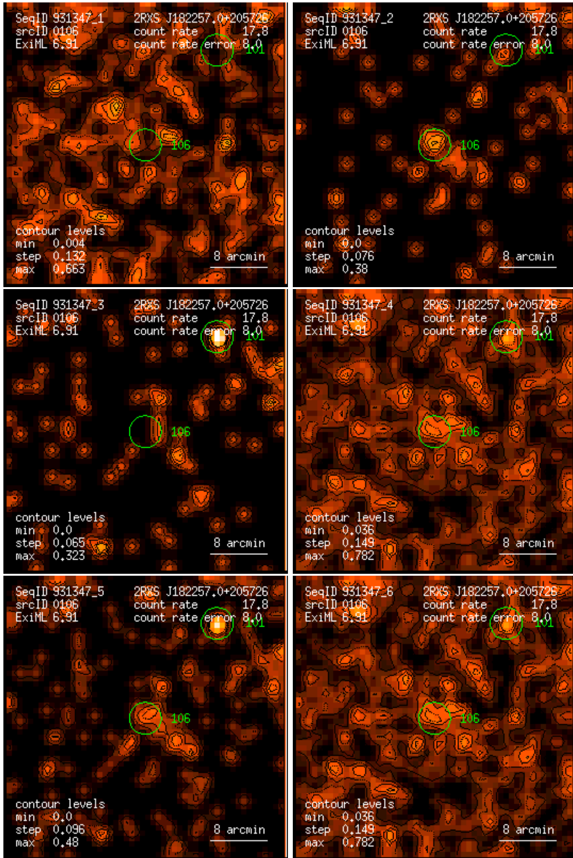
Figure 106: RASS 931347: detection 0106: band rate images, Gaussian filter: (1) PSPC channels 11 – 41, (2) 52 – 90, (3) 91 – 201, (4) 11 – 235, (5) 52 – 201, (6) 11 – 201. Broad band rates in counts/ks. Band rate contour levels in counts/ks/arcmin 2 .
