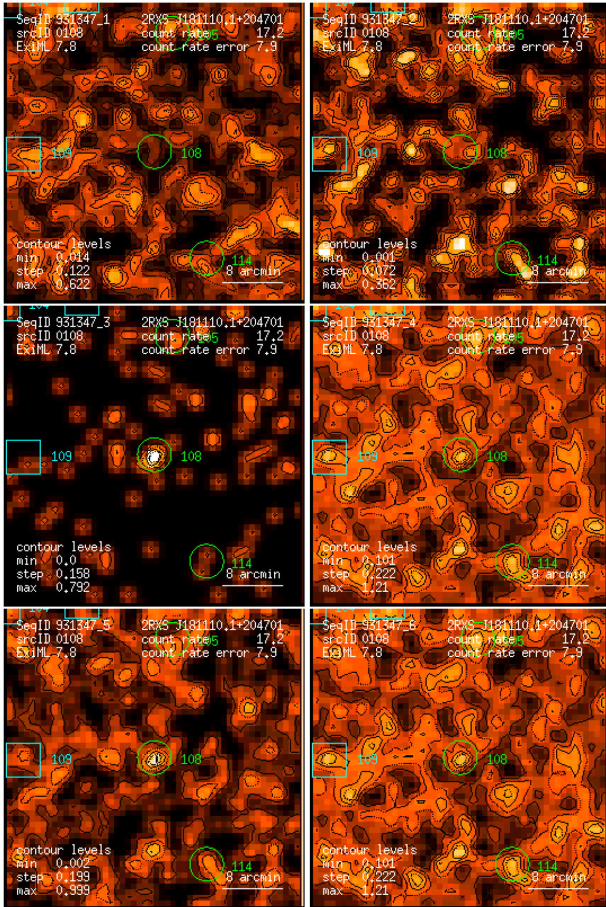
Figure 108: RASS 931347: detection 0108: band rate images, Gaussian filter: (1) PSPC channels 11 – 41, (2) 52 – 90, (3) 91 – 201, (4) 11 – 235, (5) 52 – 201, (6) 11 – 201. Broad band rates in counts/ks. Band rate contour levels in counts/ks/arcmin 2 .
