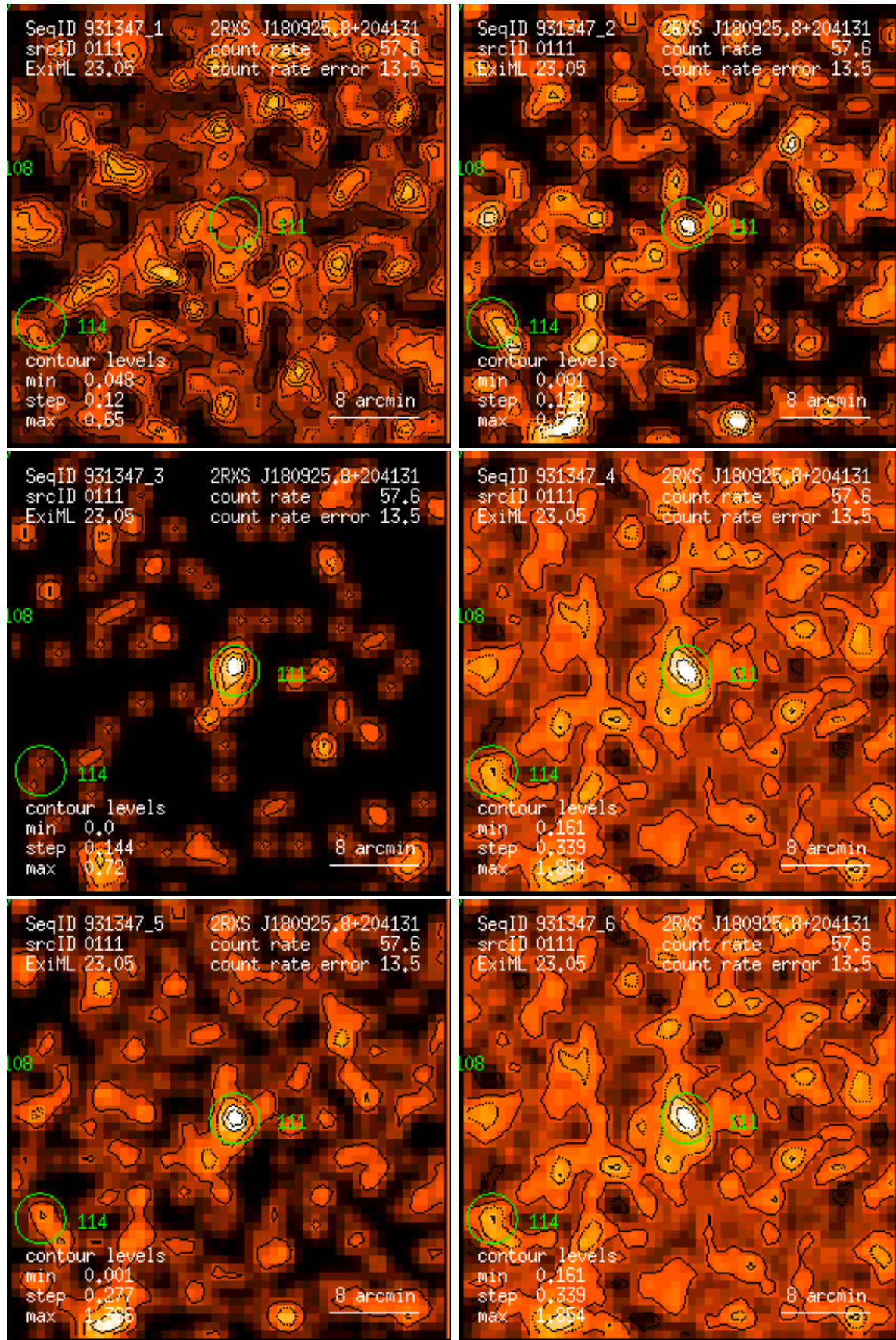
Figure 111: RASS 931347: detection 0111: band rate images, Gaussian filter: (1) PSPC channels 11 – 41, (2) 52 – 90, (3) 91 – 201, (4) 11 – 235, (5) 52 – 201, (6) 11 – 201. Broad band rates in counts/ks. Band rate contour levels in counts/ks/arcmin 2 .
