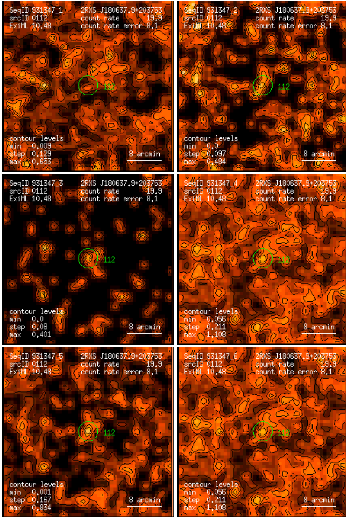
Figure 112: RASS 931347: detection 0112: band rate images, Gaussian filter: (1) PSPC channels 11 – 41, (2) 52 – 90, (3) 91 – 201, (4) 11 – 235, (5) 52 – 201, (6) 11 – 201. Broad band rates in counts/ks. Band rate contour levels in counts/ks/arcmin 2 .
