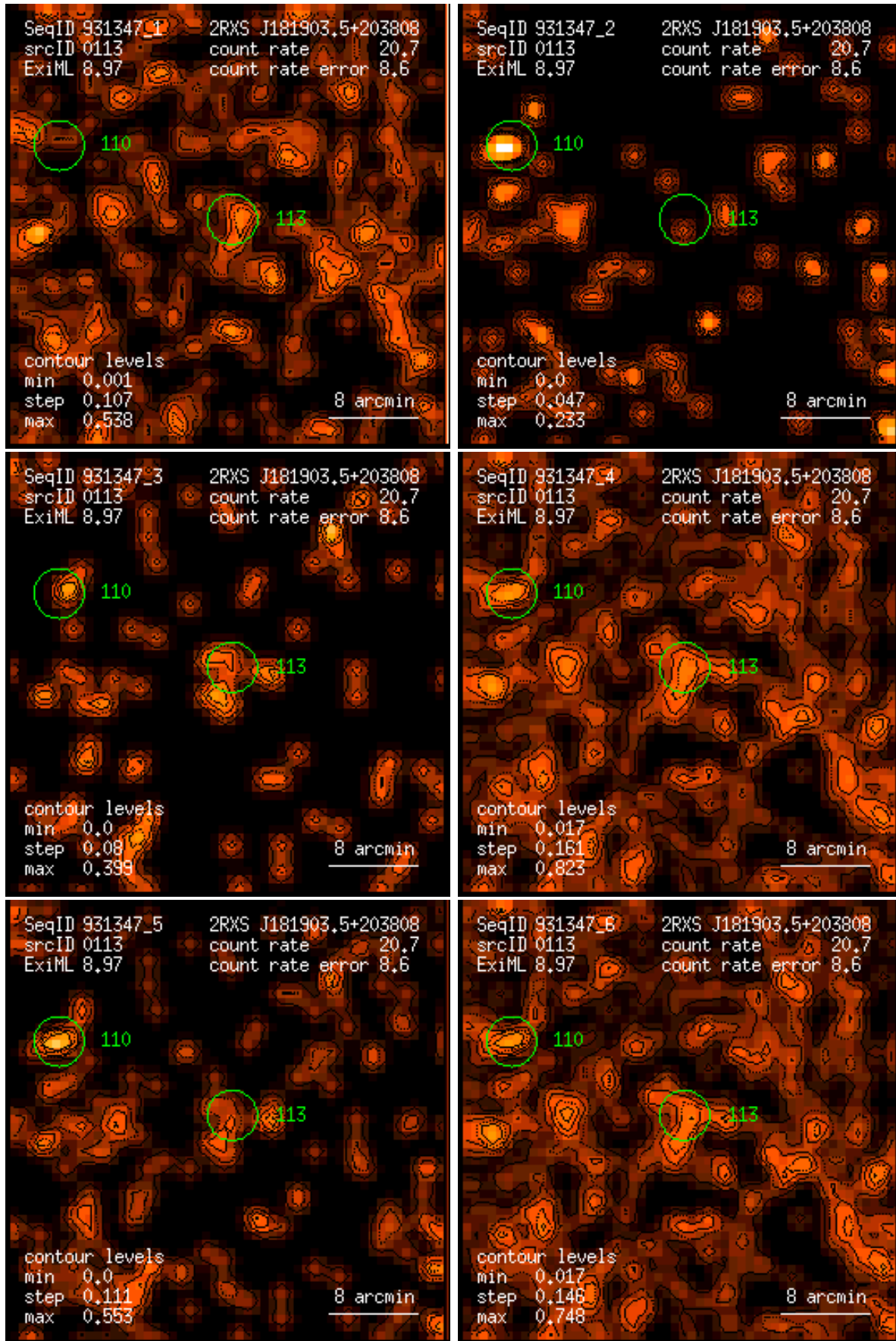
Figure 113: RASS 931347: detection 0113: band rate images, Gaussian filter: (1) PSPC channels 11 – 41, (2) 52 – 90, (3) 91 – 201, (4) 11 – 235, (5) 52 – 201, (6) 11 – 201. Broad band rates in counts/ks. Band rate contour levels in counts/ks/arcmin 2 .
