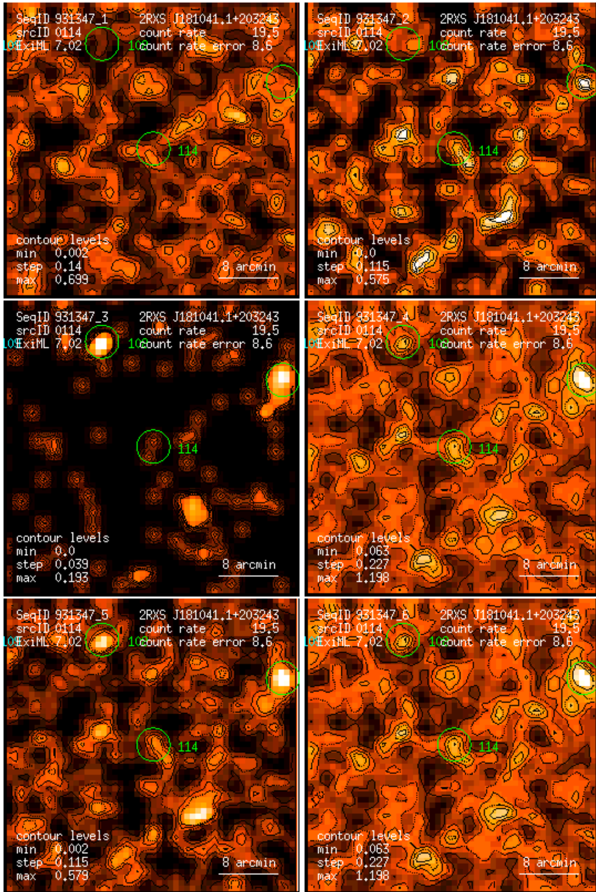
Figure 114: RASS 931347: detection 0114: band rate images, Gaussian filter: (1) PSPC channels 11 – 41, (2) 52 – 90, (3) 91 – 201, (4) 11 – 235, (5) 52 – 201, (6) 11 – 201. Broad band rates in counts/ks. Band rate contour levels in counts/ks/arcmin 2 .
